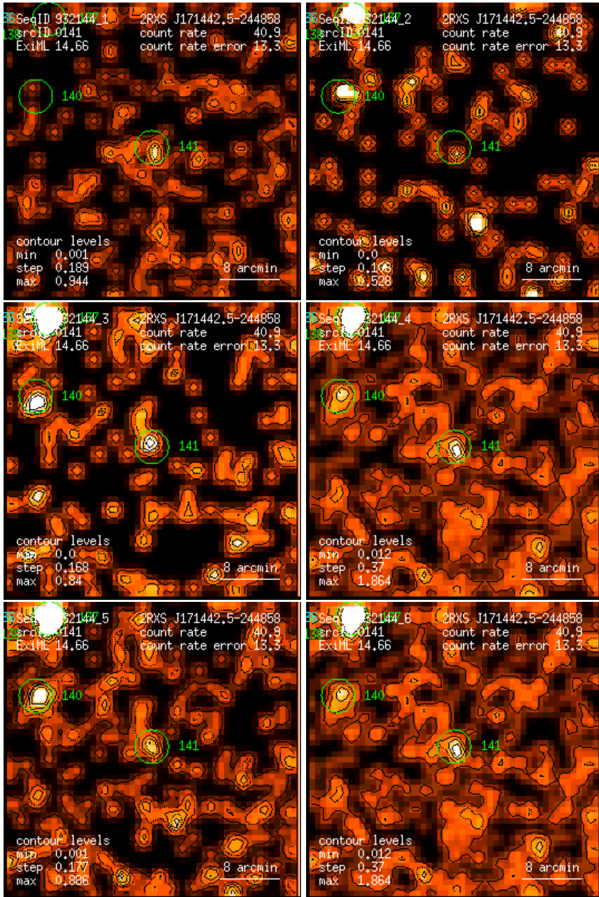
Figure 141: RASS 932144: detection 0141: band rate images, Gaussian filter: (1) PSPC channels 11 – 41, (2) 52 – 90, (3) 91 – 201, (4) 11 – 235, (5) 52 – 201, (6) 11 – 201. Broad band rates in counts/ks. Band rate contour levels in counts/ks/arcmin 2 .
