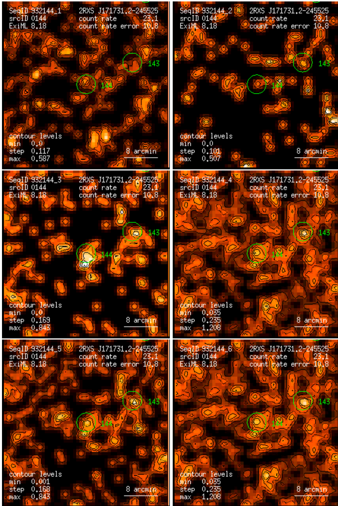
Figure 144: RASS 932144: detection 0144: band rate images, Gaussian filter: (1) PSPC channels 11 – 41, (2) 52 – 90, (3) 91 – 201, (4) 11 – 235, (5) 52 – 201, (6) 11 – 201. Broad band rates in counts/ks. Band rate contour levels in counts/ks/arcmin 2 .
