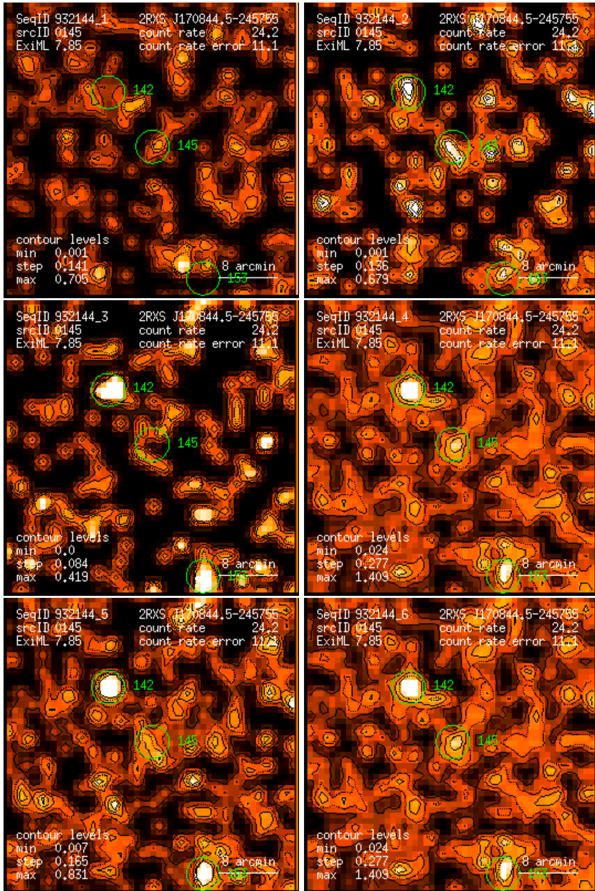
Figure 145: RASS 932144: detection 0145: band rate images, Gaussian filter: (1) PSPC channels 11 – 41, (2) 52 – 90, (3) 91 – 201, (4) 11 – 235, (5) 52 – 201, (6) 11 – 201. Broad band rates in counts/ks. Band rate contour levels in counts/ks/arcmin 2 .
