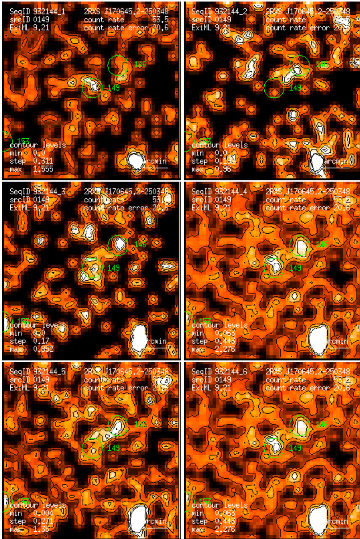
Figure 149: RASS 932144: detection 0149: band rate images, Gaussian filter: (1) PSPC channels 11 – 41, (2) 52 – 90, (3) 91 – 201, (4) 11 – 235, (5) 52 – 201, (6) 11 – 201. Broad band rates in counts/ks. Band rate contour levels in counts/ks/arcmin 2 .
