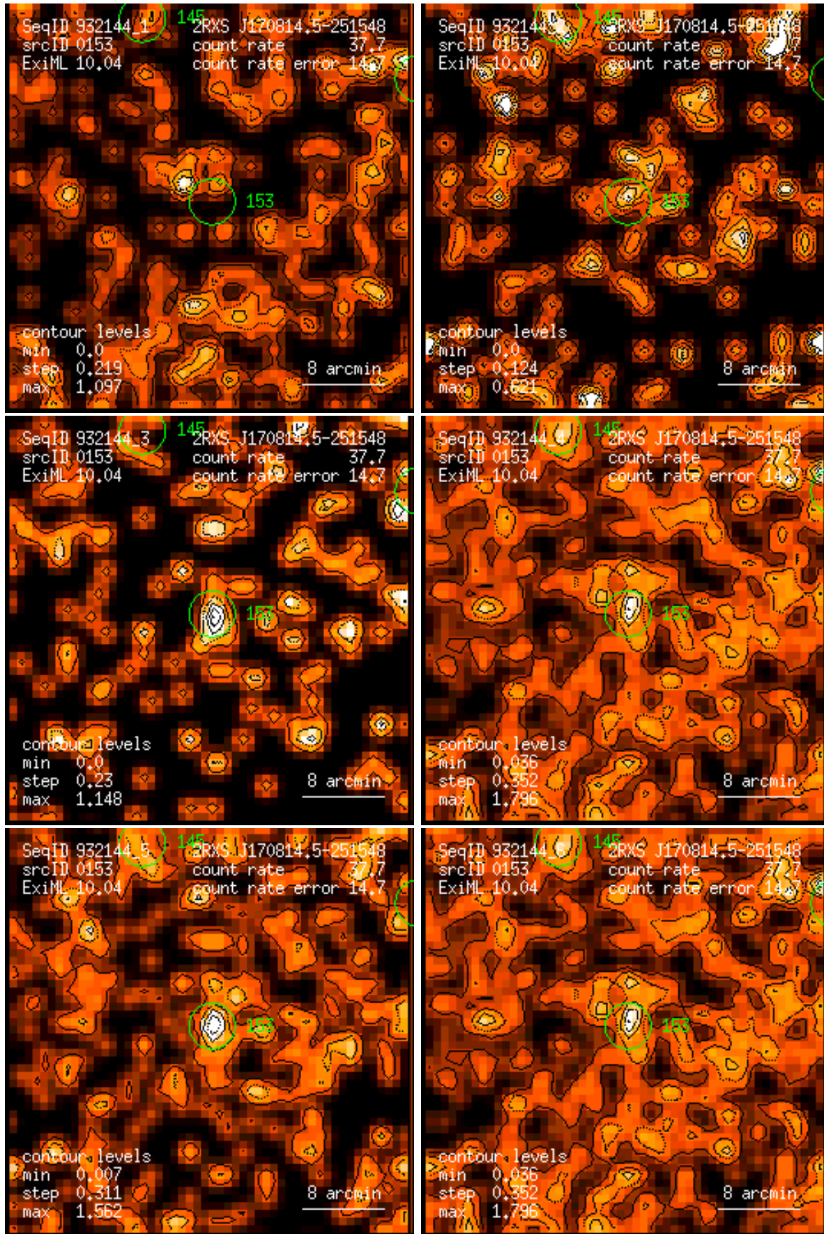
Figure 153: RASS 932144: detection 0153: band rate images, Gaussian filter: (1) PSPC channels 11 – 41, (2) 52 – 90, (3) 91 – 201, (4) 11 – 235, (5) 52 – 201, (6) 11 – 201. Broad band rates in counts/ks. Band rate contour levels in counts/ks/arcmin 2 .
