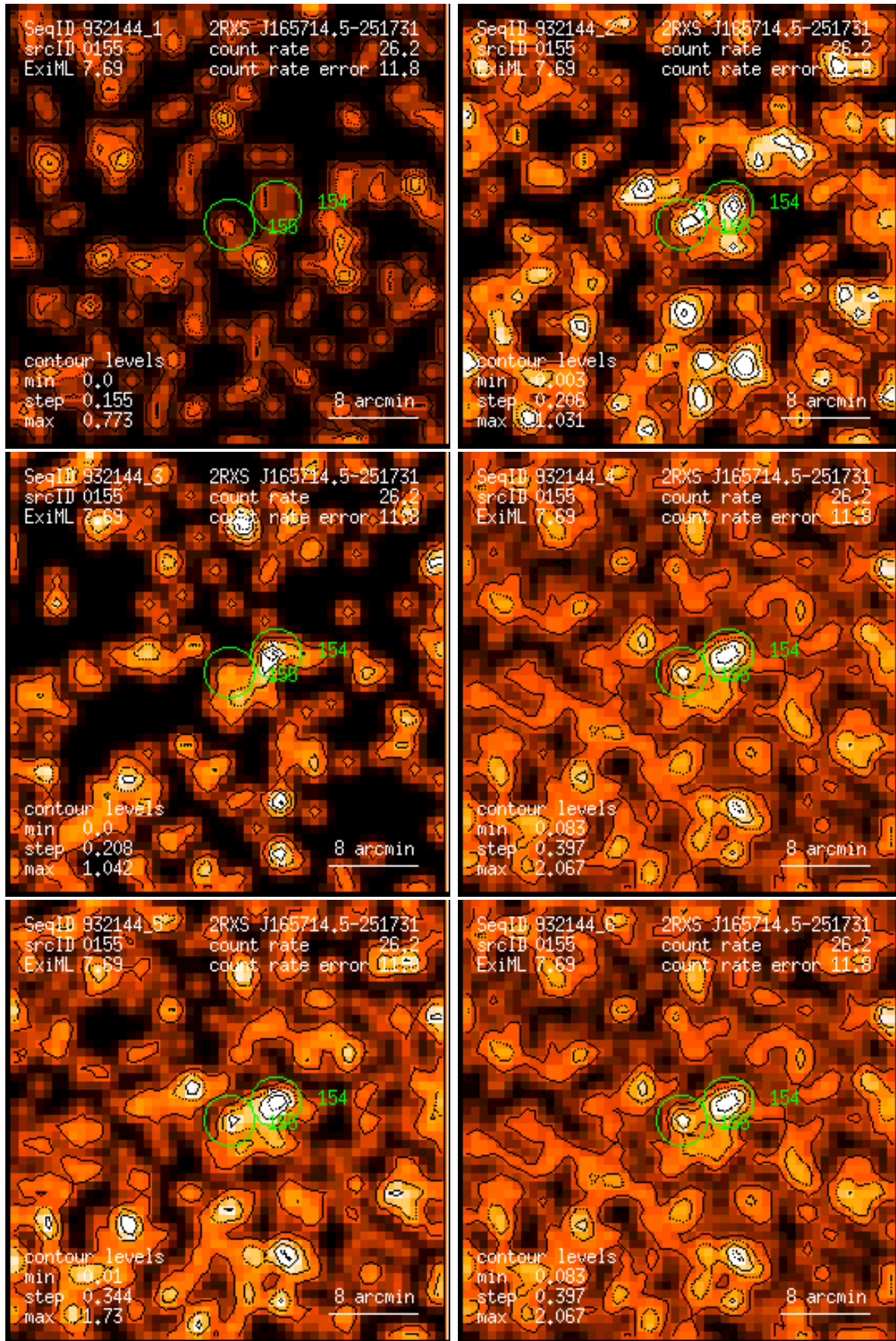
Figure 155: RASS 932144: detection 0155: band rate images, Gaussian filter: (1) PSPC channels 11 – 41, (2) 52 – 90, (3) 91 – 201, (4) 11 – 235, (5) 52 – 201, (6) 11 – 201. Broad band rates in counts/ks. Band rate contour levels in counts/ks/arcmin 2 .
