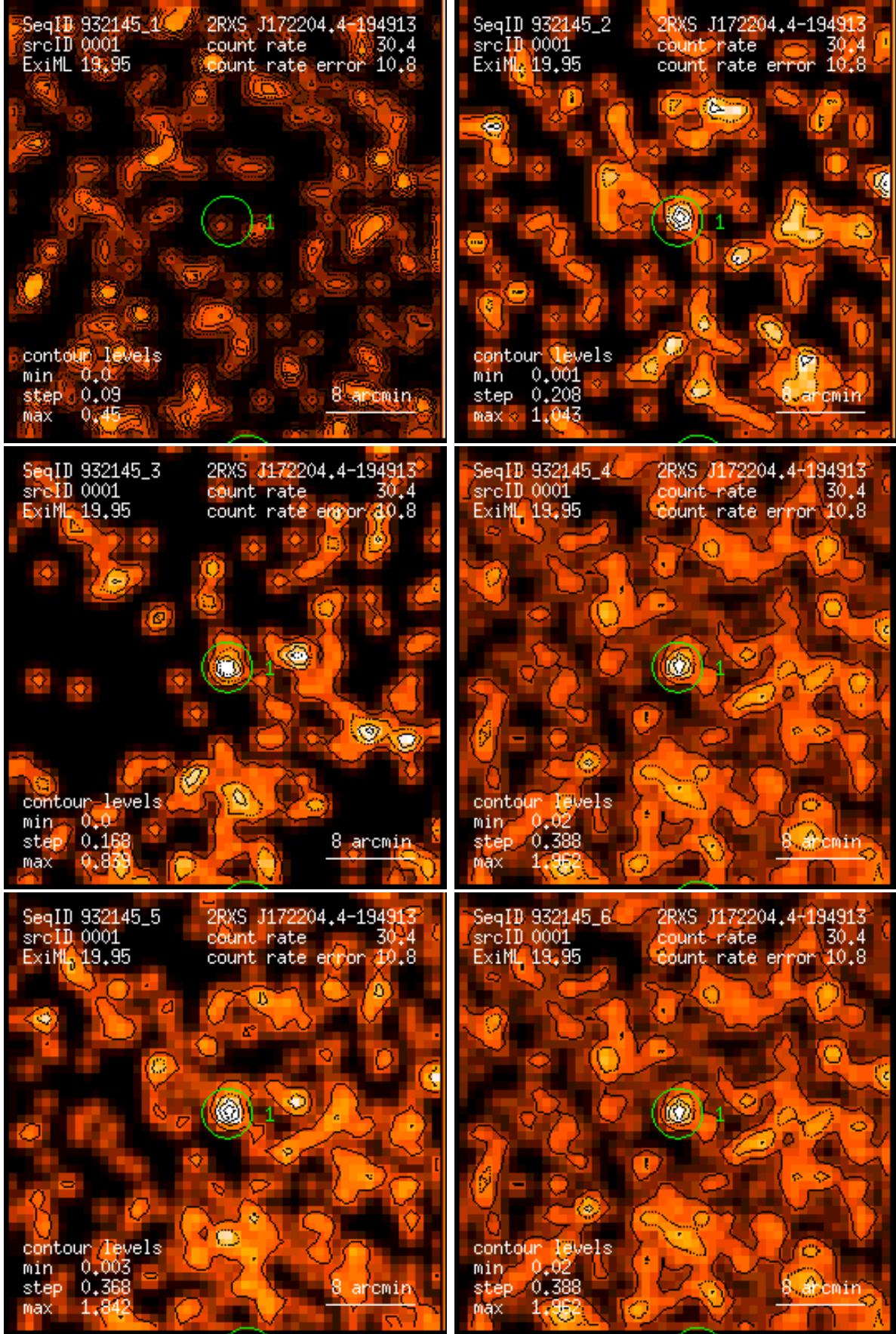
Figure 1: RASS 932145: detection 0001: band rate images, Gaussian filter: (1) PSPC channels 11 – 41, (2) 52 – 90, (3) 91 – 201, (4) 11 – 235, (5) 52 – 201, (6) 11 – 201. Broad band rates in counts/ks. Band rate contour levels in counts/ks/arcmin 2 .
