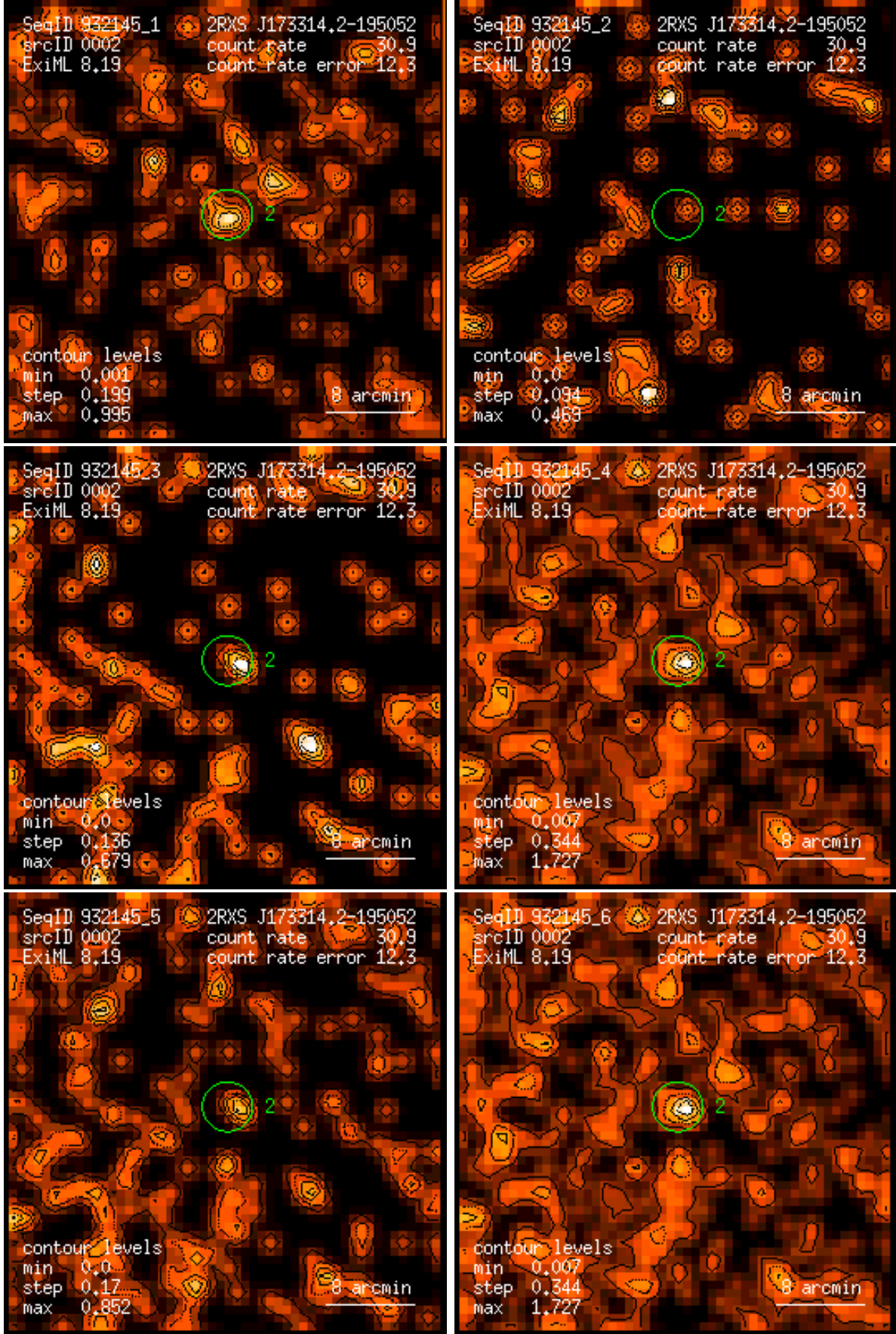
Figure 2: RASS 932145: detection 0002: band rate images, Gaussian filter: (1) PSPC channels 11 – 41, (2) 52 – 90, (3) 91 – 201, (4) 11 – 235, (5) 52 – 201, (6) 11 – 201. Broad band rates in counts/ks. Band rate contour levels in counts/ks/arcmin 2 .
