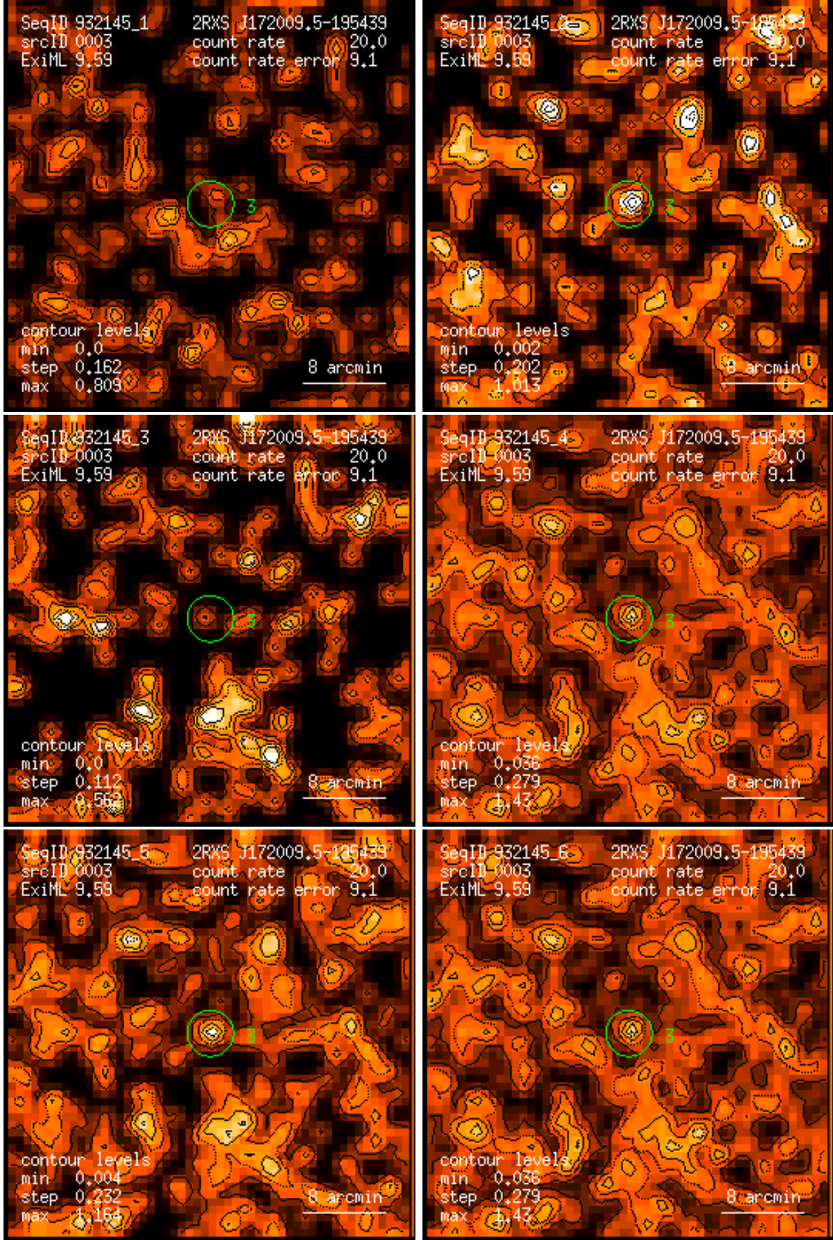
Figure 3: RASS 932145: detection 0003: band rate images, Gaussian filter: (1) PSPC channels 11 – 41, (2) 52 – 90, (3) 91 – 201, (4) 11 – 235, (5) 52 – 201, (6) 11 – 201. Broad band rates in counts/ks. Band rate contour levels in counts/ks/arcmin 2 .
