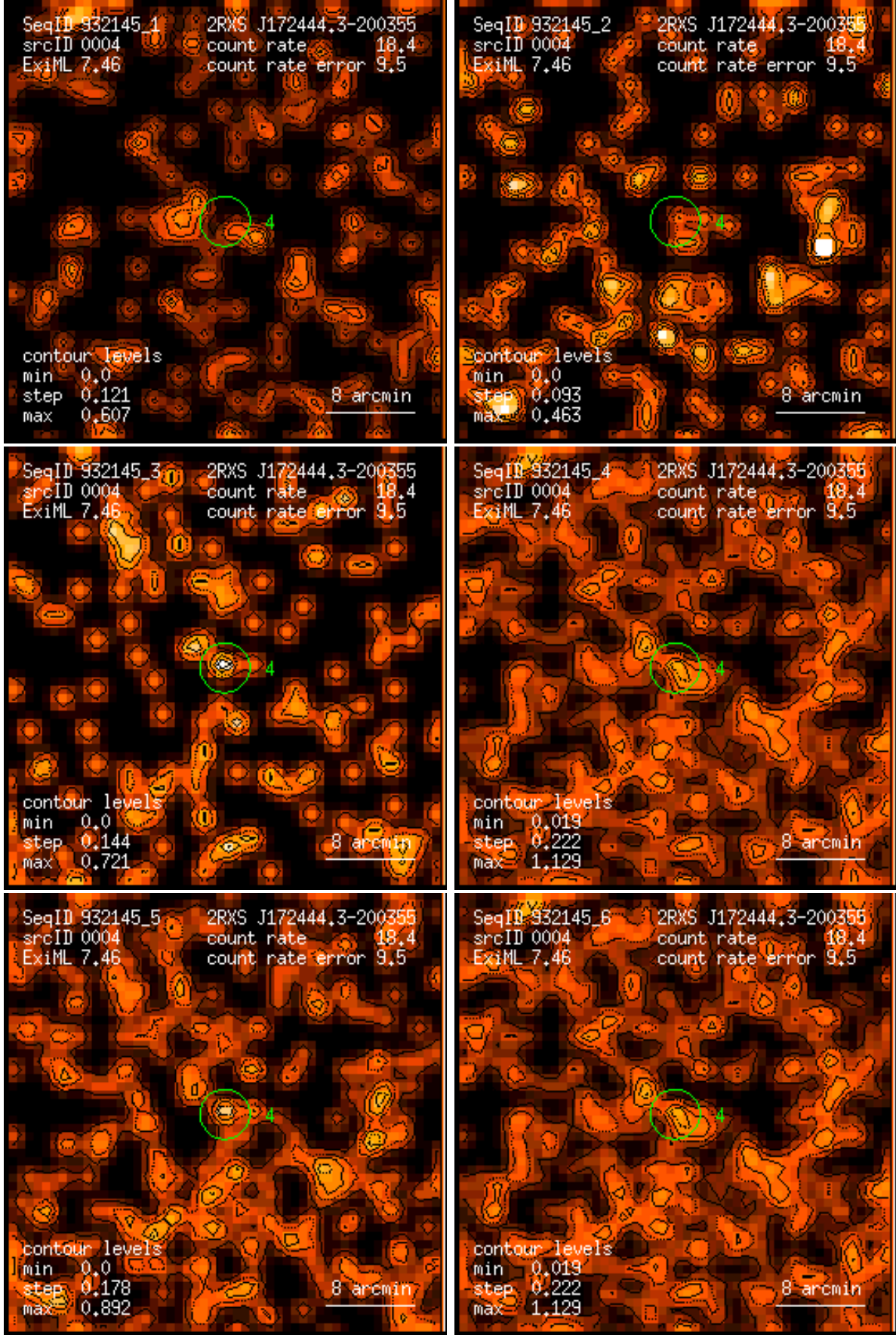
Figure 4: RASS 932145: detection 0004: band rate images, Gaussian filter: (1) PSPC channels 11 – 41, (2) 52 – 90, (3) 91 – 201, (4) 11 – 235, (5) 52 – 201, (6) 11 – 201. Broad band rates in counts/ks. Band rate contour levels in counts/ks/arcmin 2 .
