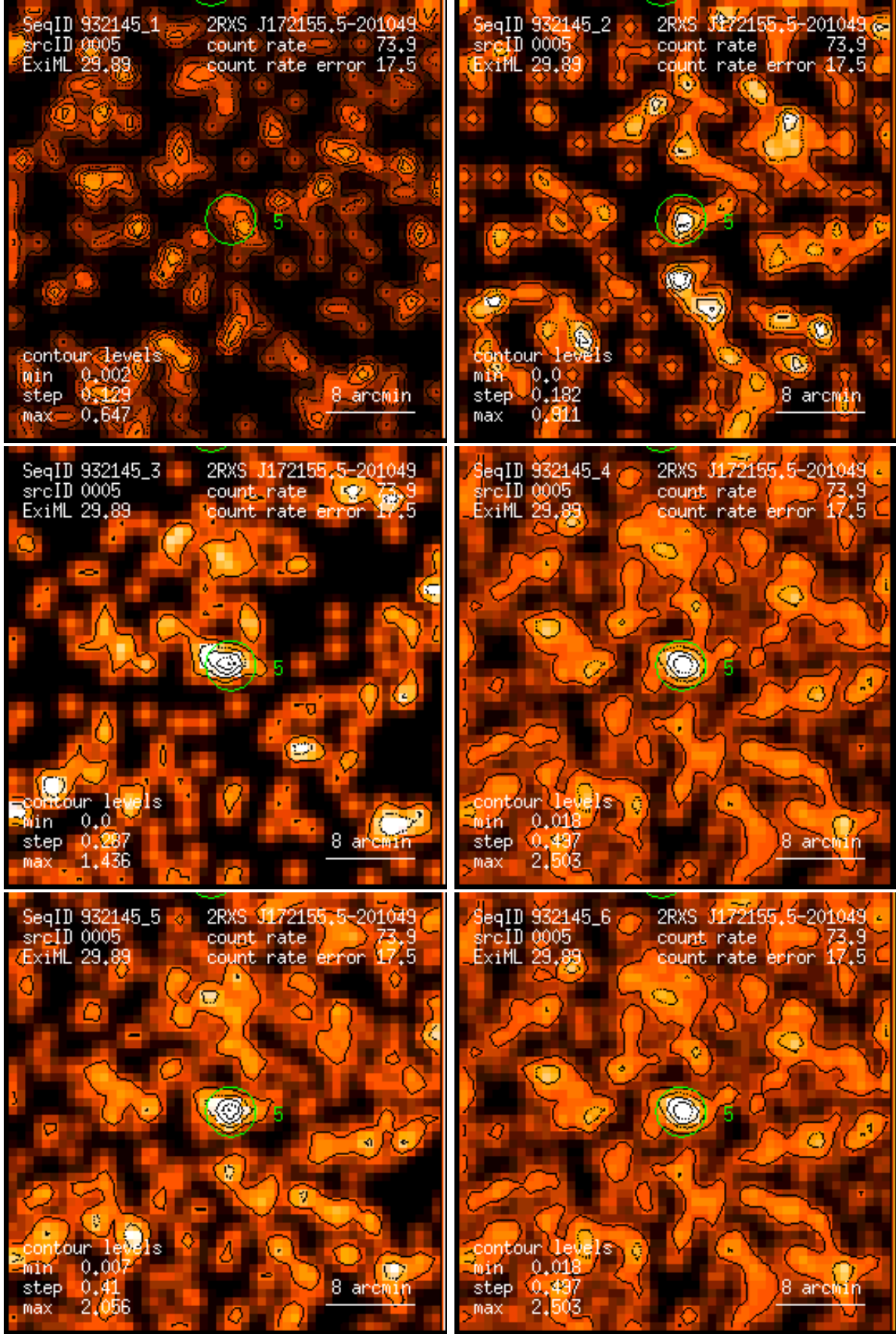
Figure 5: RASS 932145: detection 0005: band rate images, Gaussian filter: (1) PSPC channels 11 – 41, (2) 52 – 90, (3) 91 – 201, (4) 11 – 235, (5) 52 – 201, (6) 11 – 201. Broad band rates in counts/ks. Band rate contour levels in counts/ks/arcmin 2 .
