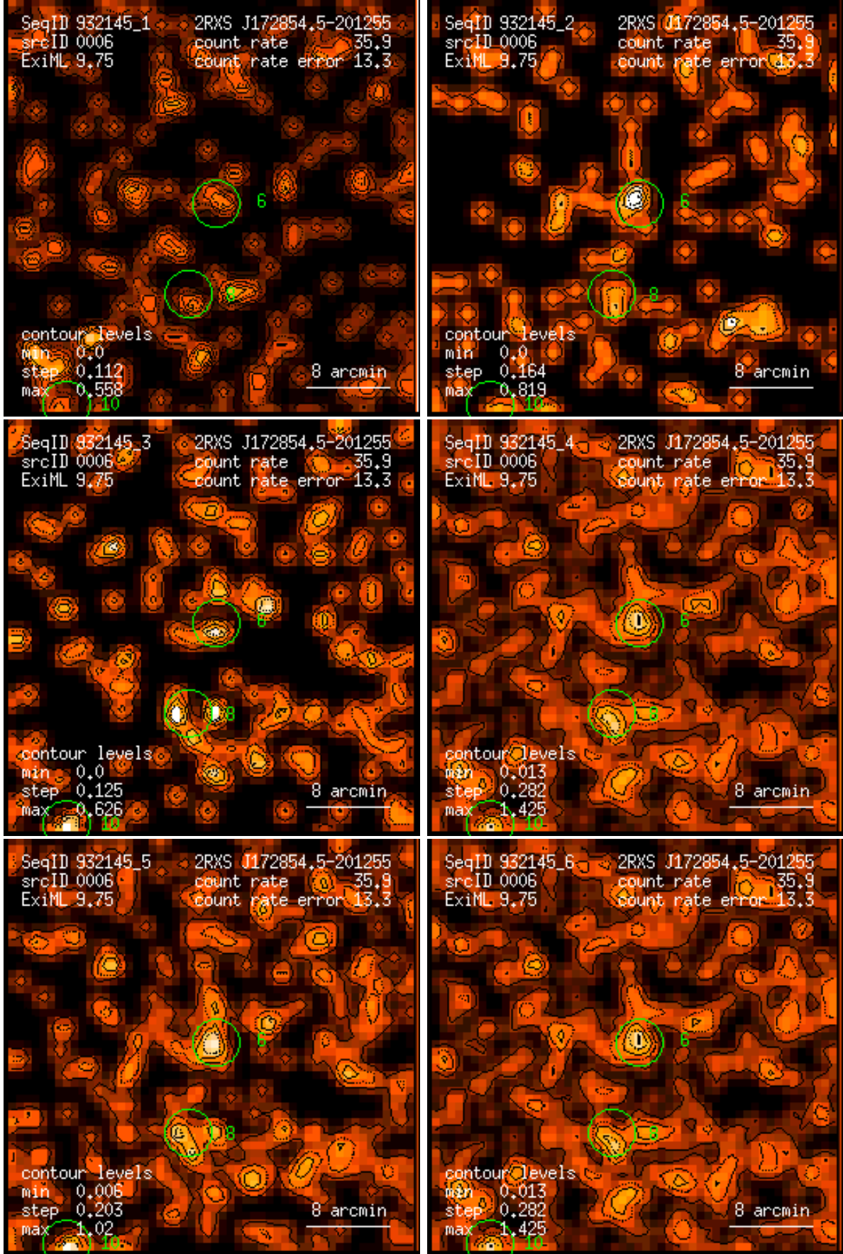
Figure 6: RASS 932145: detection 0006: band rate images, Gaussian filter: (1) PSPC channels 11 – 41, (2) 52 – 90, (3) 91 – 201, (4) 11 – 235, (5) 52 – 201, (6) 11 – 201. Broad band rates in counts/ks. Band rate contour levels in counts/ks/arcmin 2 .
