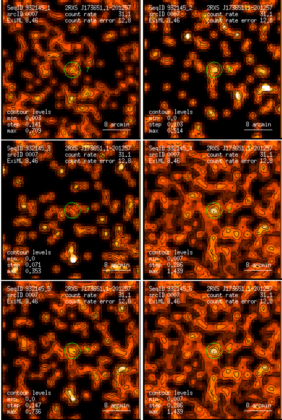
Figure 7: RASS 932145: detection 0007: band rate images, Gaussian filter: (1) PSPC channels 11 – 41, (2) 52 – 90, (3) 91 – 201, (4) 11 – 235, (5) 52 – 201, (6) 11 – 201. Broad band rates in counts/ks. Band rate contour levels in counts/ks/arcmin 2 .
