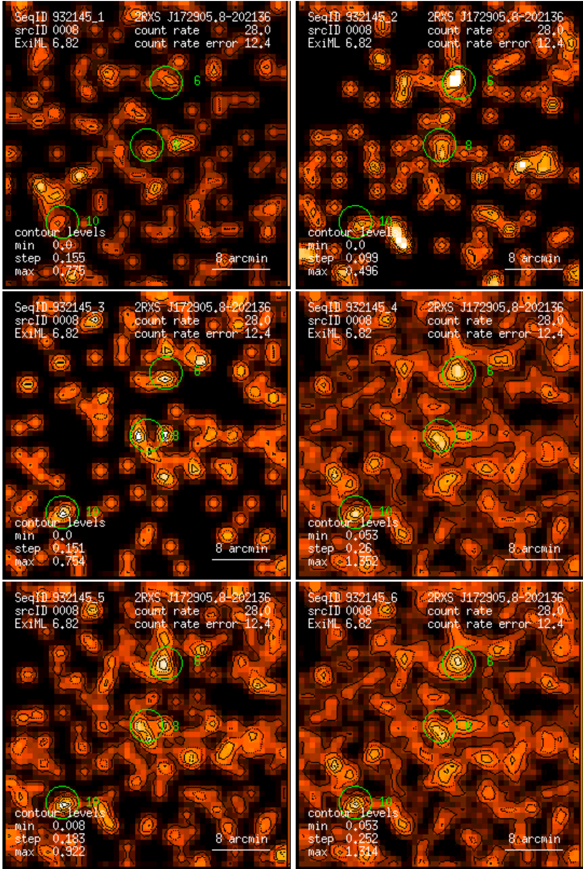
Figure 8: RASS 932145: detection 0008: band rate images, Gaussian filter: (1) PSPC channels 11 – 41, (2) 52 – 90, (3) 91 – 201, (4) 11 – 235, (5) 52 – 201, (6) 11 – 201. Broad band rates in counts/ks. Band rate contour levels in counts/ks/arcmin 2 .
