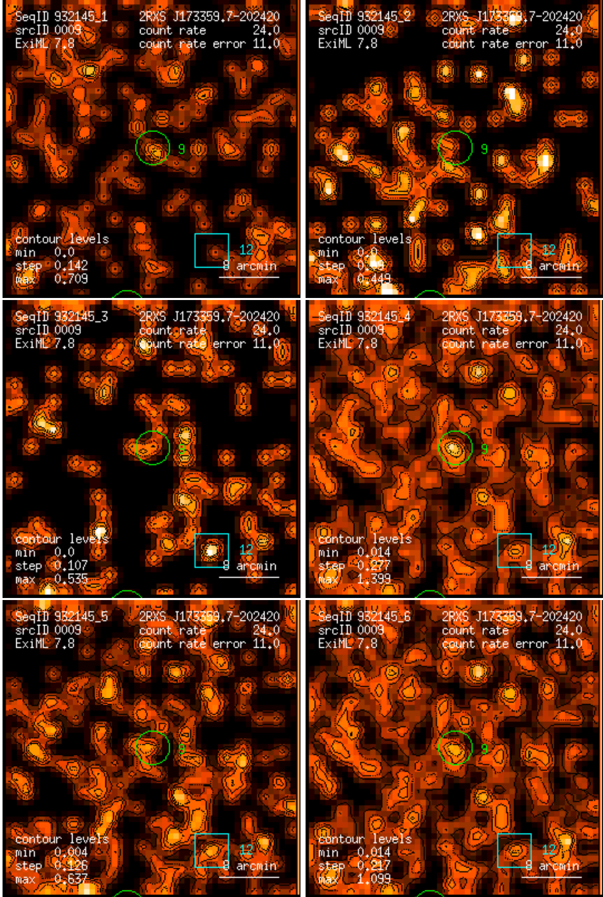
Figure 9: RASS 932145: detection 0009: band rate images, Gaussian filter: (1) PSPC channels 11 – 41, (2) 52 – 90, (3) 91 – 201, (4) 11 – 235, (5) 52 – 201, (6) 11 – 201. Broad band rates in counts/ks. Band rate contour levels in counts/ks/arcmin 2 .
