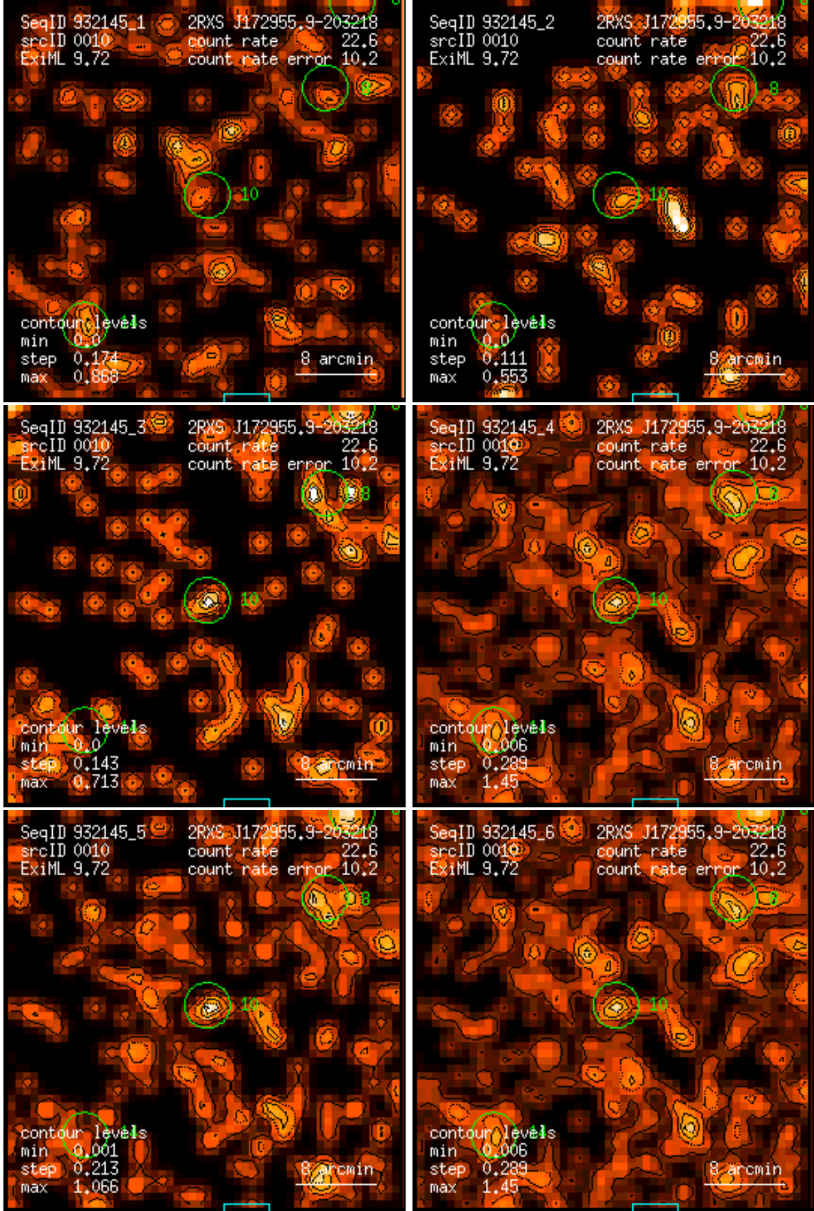
Figure 10: RASS 932145: detection 0010: band rate images, Gaussian filter: (1) PSPC channels 11 – 41, (2) 52 – 90, (3) 91 – 201, (4) 11 – 235, (5) 52 – 201, (6) 11 – 201. Broad band rates in counts/ks. Band rate contour levels in counts/ks/arcmin 2 .
