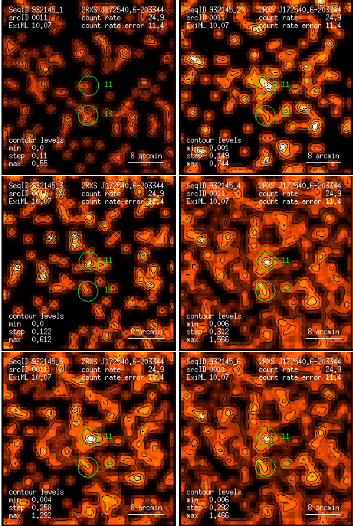
Figure 11: RASS 932145: detection 0011: band rate images, Gaussian filter: (1) PSPC channels 11 – 41, (2) 52 – 90, (3) 91 – 201, (4) 11 – 235, (5) 52 – 201, (6) 11 – 201. Broad band rates in counts/ks. Band rate contour levels in counts/ks/arcmin 2 .
