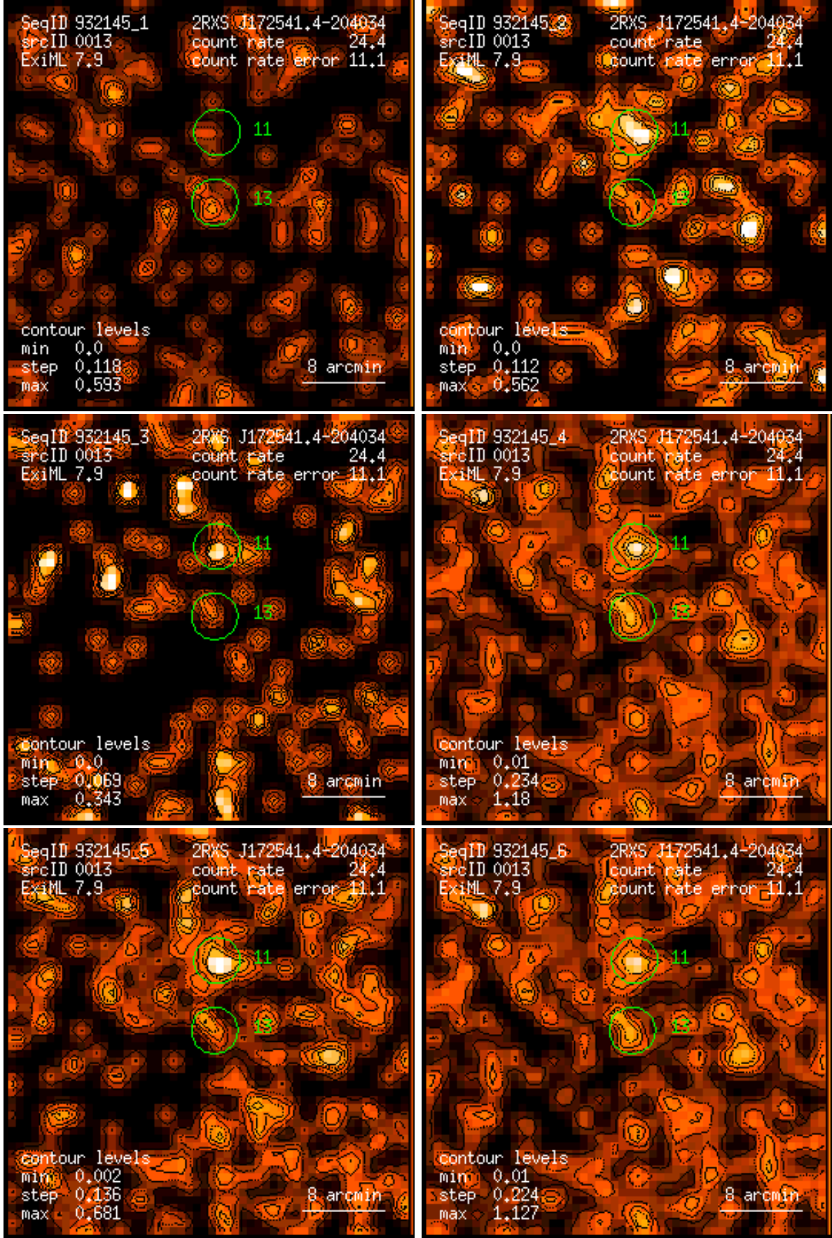
Figure 13: RASS 932145: detection 0013: band rate images, Gaussian filter: (1) PSPC channels 11 – 41, (2) 52 – 90, (3) 91 – 201, (4) 11 – 235, (5) 52 – 201, (6) 11 – 201. Broad band rates in counts/ks. Band rate contour levels in counts/ks/arcmin 2 .
