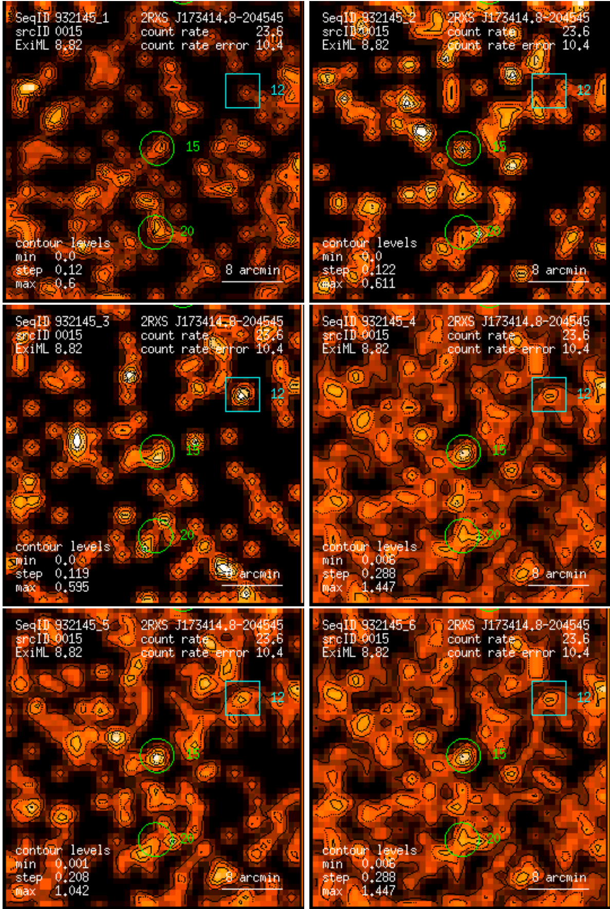
Figure 15: RASS 932145: detection 0015: band rate images, Gaussian filter: (1) PSPC channels 11 – 41, (2) 52 – 90, (3) 91 – 201, (4) 11 – 235, (5) 52 – 201, (6) 11 – 201. Broad band rates in counts/ks. Band rate contour levels in counts/ks/arcmin 2 .
