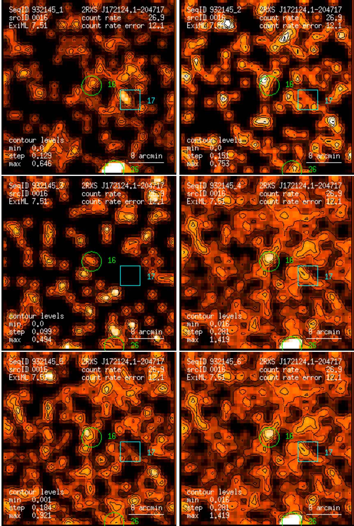
Figure 16: RASS 932145: detection 0016: band rate images, Gaussian filter: (1) PSPC channels 11 – 41, (2) 52 – 90, (3) 91 – 201, (4) 11 – 235, (5) 52 – 201, (6) 11 – 201. Broad band rates in counts/ks. Band rate contour levels in counts/ks/arcmin 2 .
