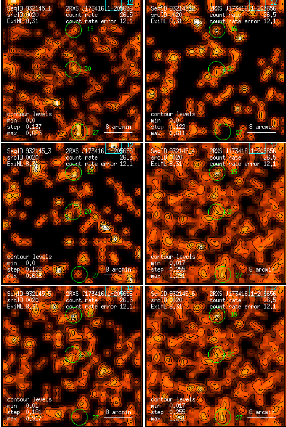
Figure 20: RASS 932145: detection 0020: band rate images, Gaussian filter: (1) PSPC channels 11 – 41, (2) 52 – 90, (3) 91 – 201, (4) 11 – 235, (5) 52 – 201, (6) 11 – 201. Broad band rates in counts/ks. Band rate contour levels in counts/ks/arcmin 2 .
