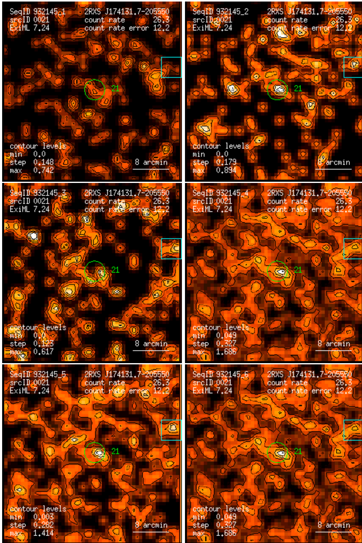
Figure 21: RASS 932145: detection 0021: band rate images, Gaussian filter: (1) PSPC channels 11 – 41, (2) 52 – 90, (3) 91 – 201, (4) 11 – 235, (5) 52 – 201, (6) 11 – 201. Broad band rates in counts/ks. Band rate contour levels in counts/ks/arcmin 2 .
