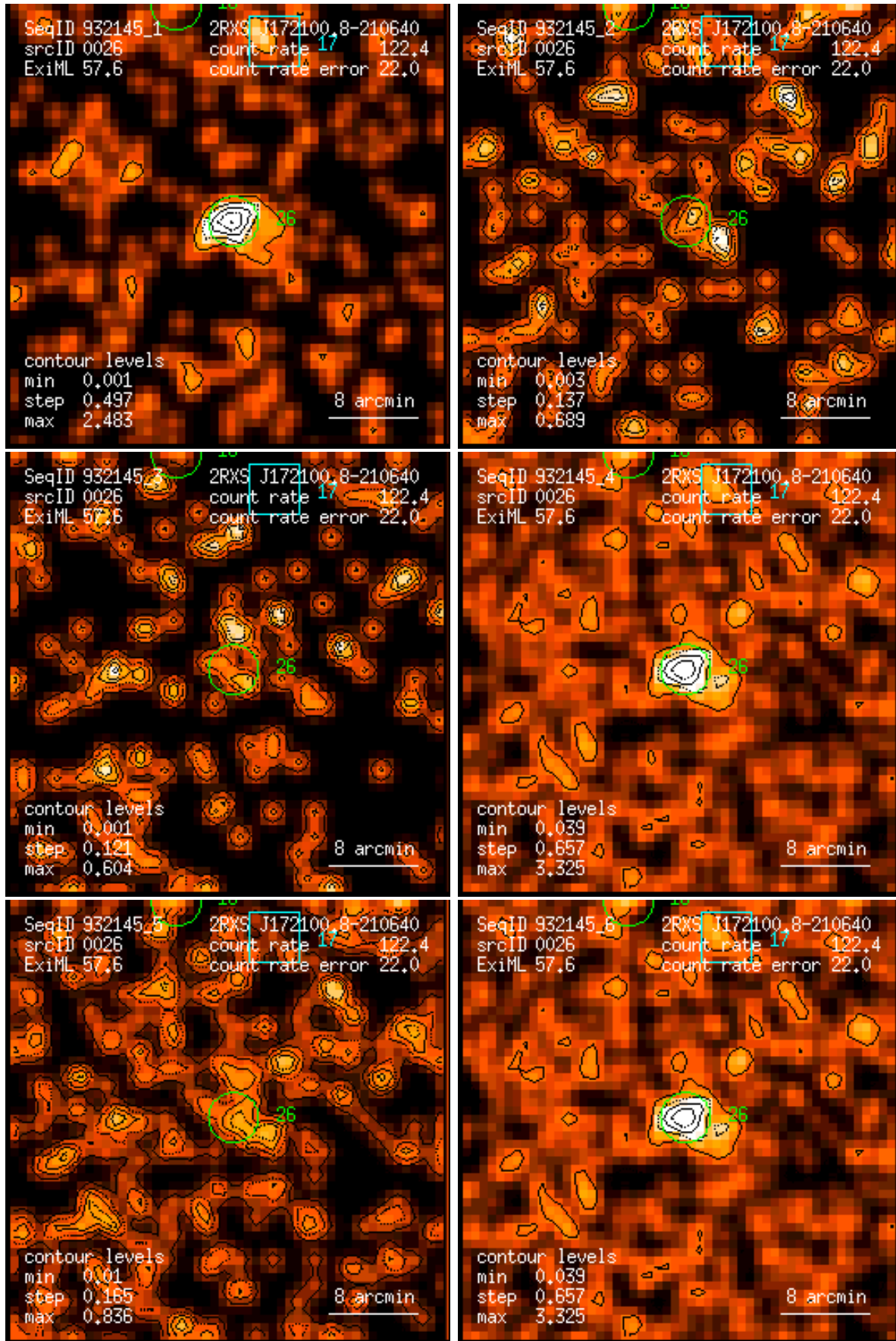
Figure 26: RASS 932145: detection 0026: band rate images, Gaussian filter: (1) PSPC channels 11 – 41, (2) 52 – 90, (3) 91 – 201, (4) 11 – 235, (5) 52 – 201, (6) 11 – 201. Broad band rates in counts/ks. Band rate contour levels in counts/ks/arcmin 2 .
