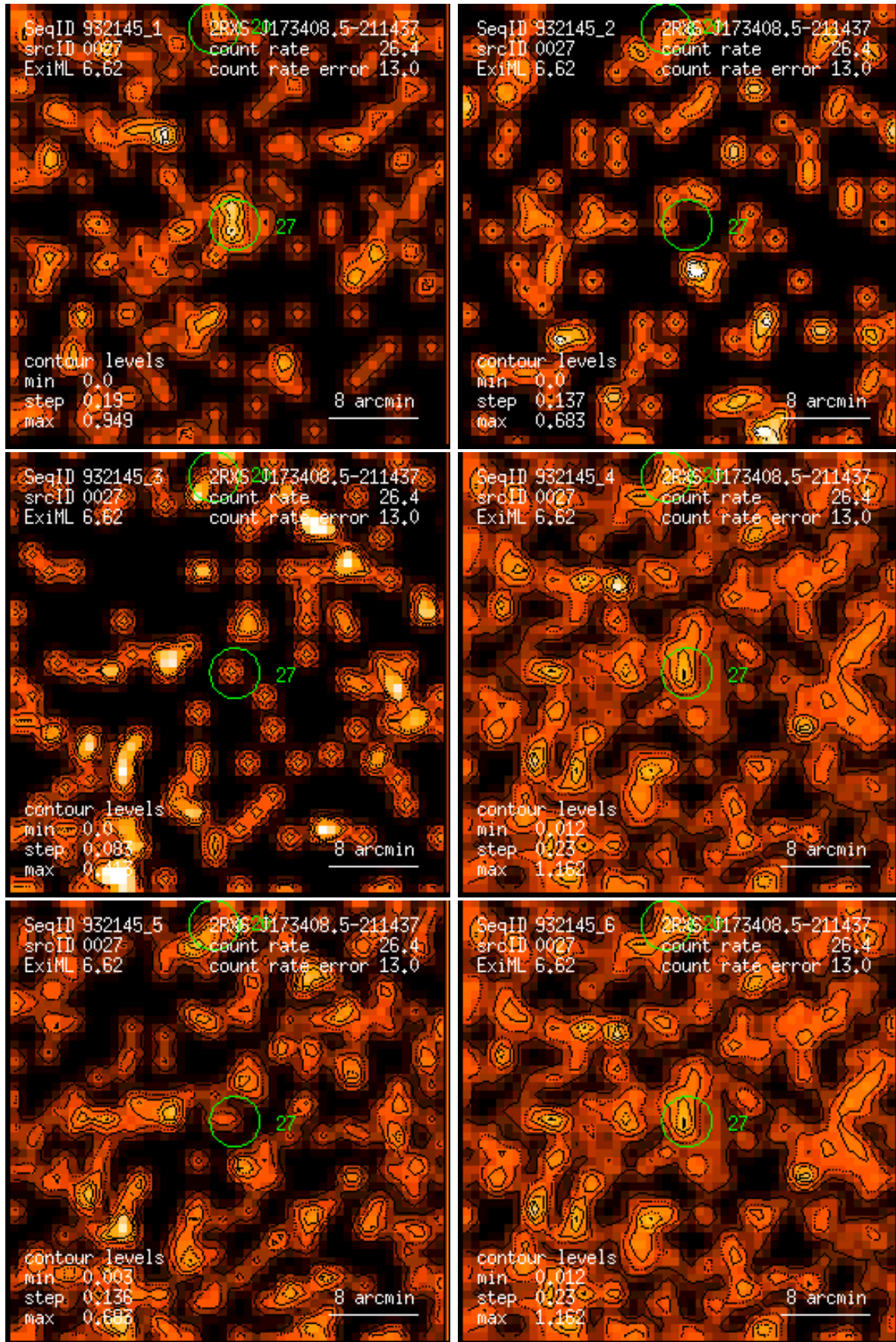
Figure 27: RASS 932145: detection 0027: band rate images, Gaussian filter: (1) PSPC channels 11 – 41, (2) 52 – 90, (3) 91 – 201, (4) 11 – 235, (5) 52 – 201, (6) 11 – 201. Broad band rates in counts/ks. Band rate contour levels in counts/ks/arcmin 2 .
