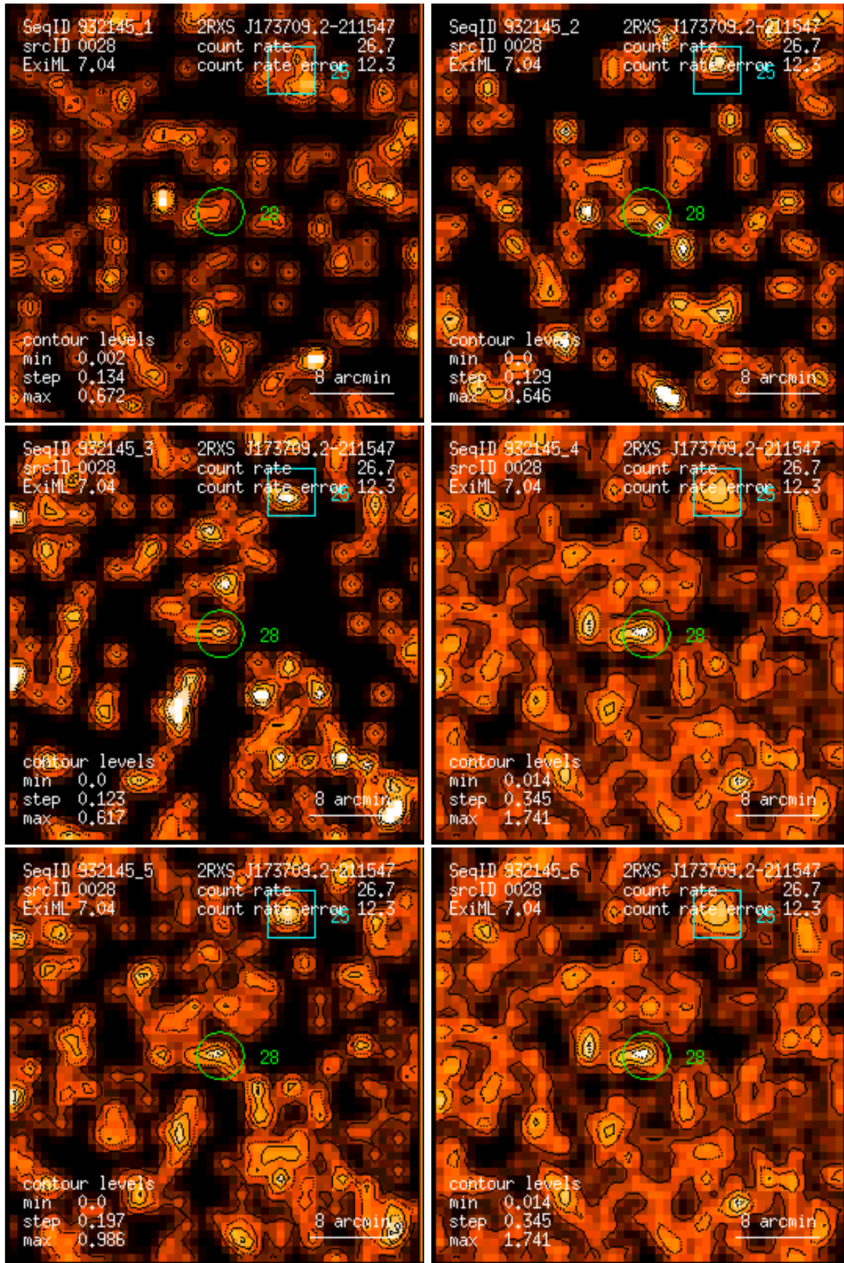
Figure 28: RASS 932145: detection 0028: band rate images, Gaussian filter: (1) PSPC channels 11 – 41, (2) 52 – 90, (3) 91 – 201, (4) 11 – 235, (5) 52 – 201, (6) 11 – 201. Broad band rates in counts/ks. Band rate contour levels in counts/ks/arcmin 2 .
