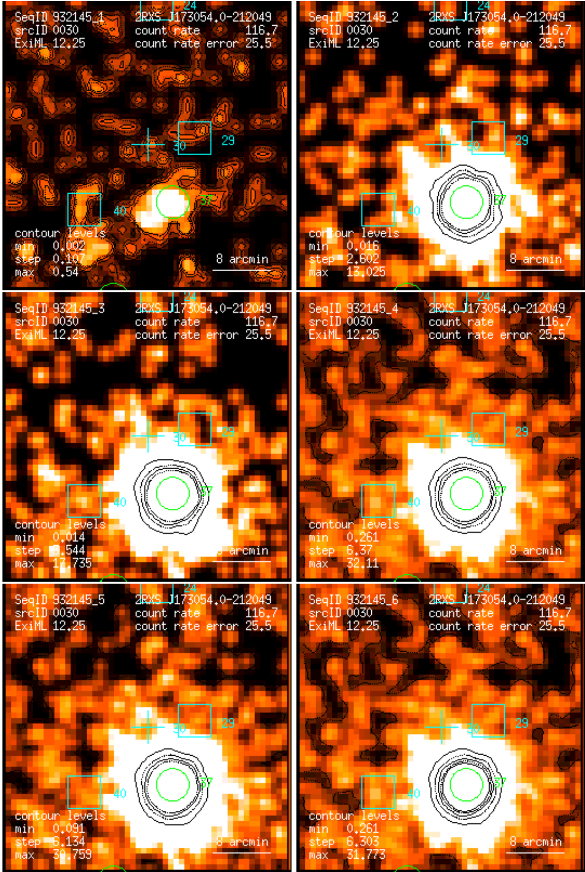
Figure 30: RASS 932145: detection 0030: band rate images, Gaussian filter: (1) PSPC channels 11 – 41, (2) 52 – 90, (3) 91 – 201, (4) 11 – 235, (5) 52 – 201, (6) 11 – 201. Broad band rates in counts/ks. Band rate contour levels in counts/ks/arcmin 2 .
