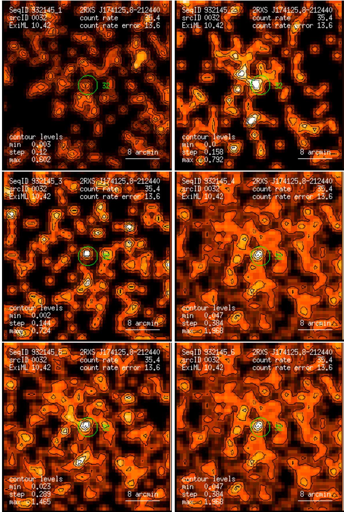
Figure 32: RASS 932145: detection 0032: band rate images, Gaussian filter: (1) PSPC channels 11 – 41, (2) 52 – 90, (3) 91 – 201, (4) 11 – 235, (5) 52 – 201, (6) 11 – 201. Broad band rates in counts/ks. Band rate contour levels in counts/ks/arcmin 2 .
