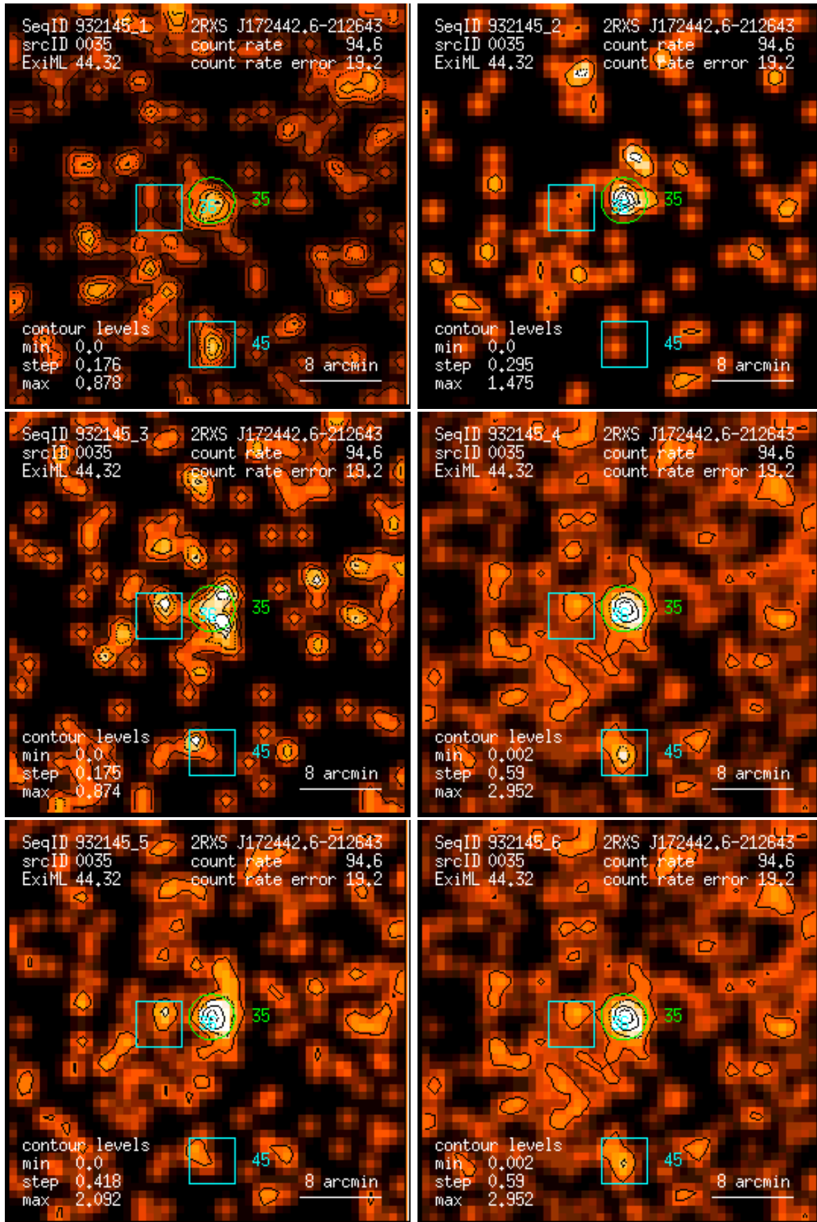
Figure 35: RASS 932145: detection 0035: band rate images, Gaussian filter: (1) PSPC channels 11 – 41, (2) 52 – 90, (3) 91 – 201, (4) 11 – 235, (5) 52 – 201, (6) 11 – 201. Broad band rates in counts/ks. Band rate contour levels in counts/ks/arcmin 2 .
