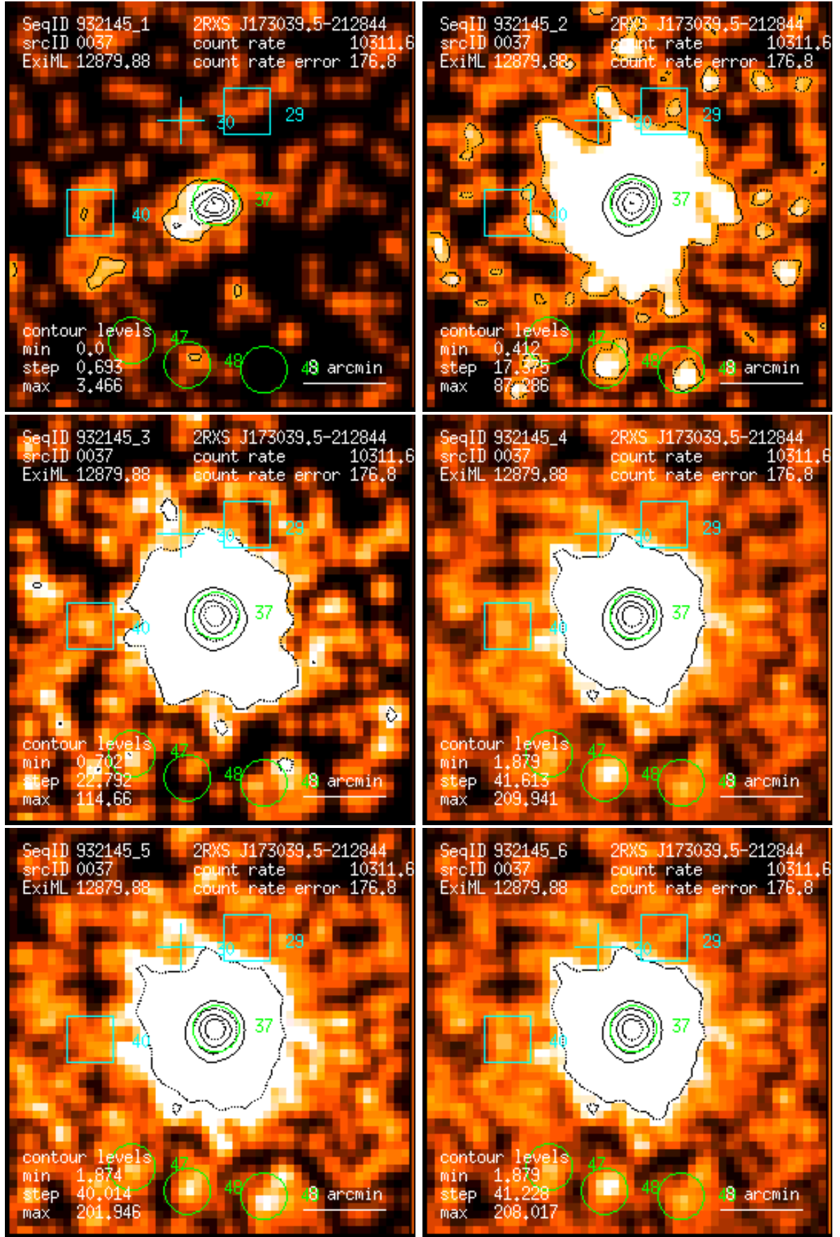
Figure 37: RASS 932145: detection 0037: band rate images, Gaussian filter: (1) PSPC channels 11 – 41, (2) 52 – 90, (3) 91 – 201, (4) 11 – 235, (5) 52 – 201, (6) 11 – 201. Broad band rates in counts/ks. Band rate contour levels in counts/ks/arcmin 2 .
