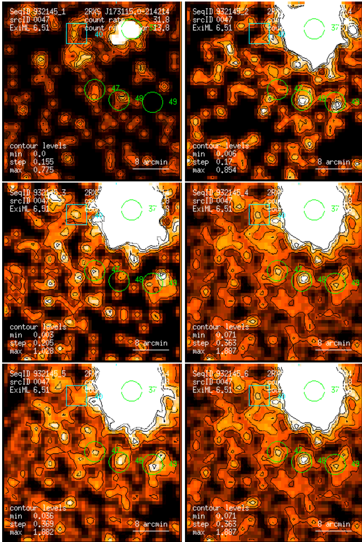
Figure 47: RASS 932145: detection 0047: band rate images, Gaussian filter: (1) PSPC channels 11 – 41, (2) 52 – 90, (3) 91 – 201, (4) 11 – 235, (5) 52 – 201, (6) 11 – 201. Broad band rates in counts/ks. Band rate contour levels in counts/ks/arcmin 2 .
