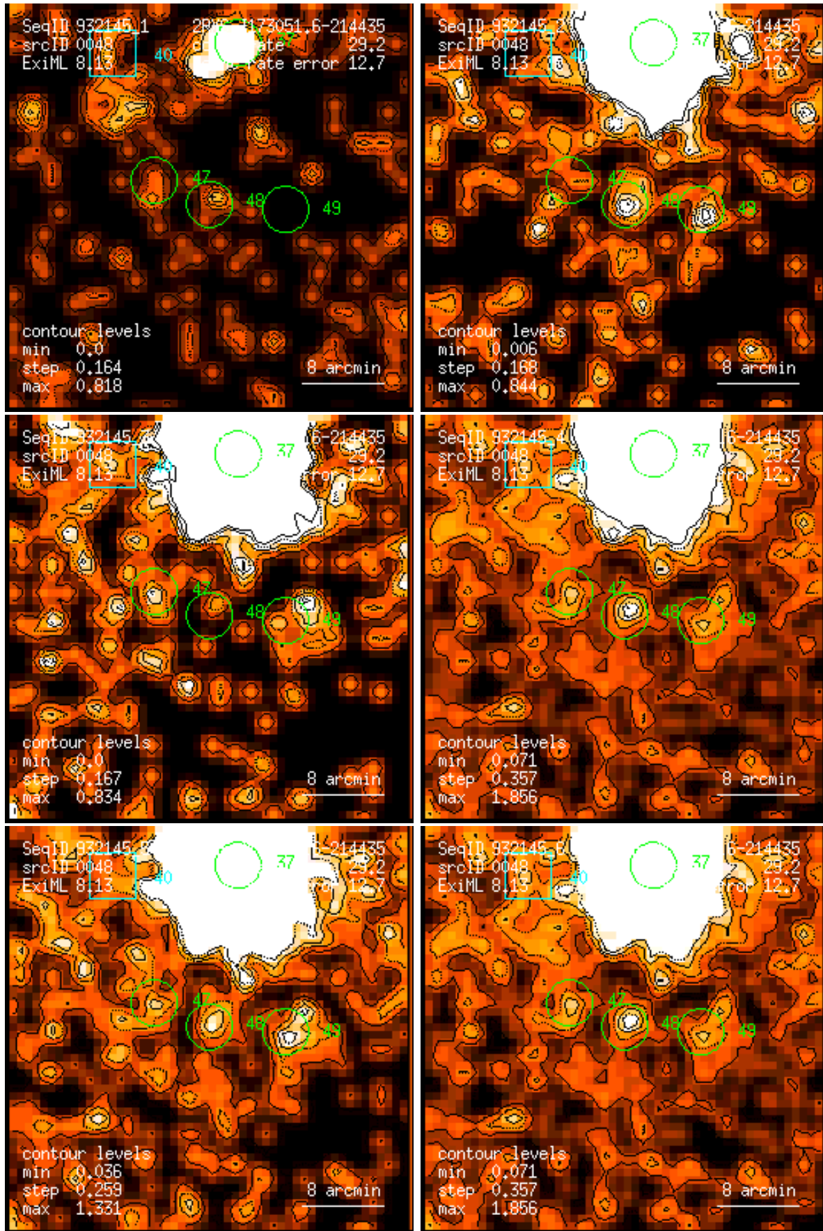
Figure 48: RASS 932145: detection 0048: band rate images, Gaussian filter: (1) PSPC channels 11 – 41, (2) 52 – 90, (3) 91 – 201, (4) 11 – 235, (5) 52 – 201, (6) 11 – 201. Broad band rates in counts/ks. Band rate contour levels in counts/ks/arcmin 2 .
