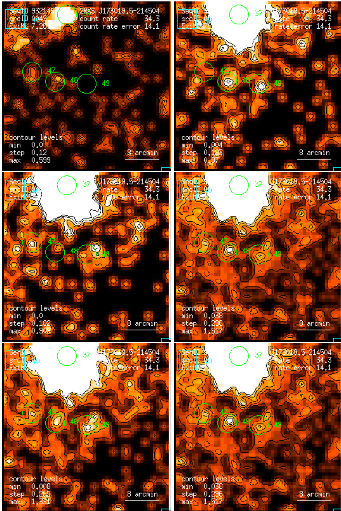
Figure 49: RASS 932145: detection 0049: band rate images, Gaussian filter: (1) PSPC channels 11 – 41, (2) 52 – 90, (3) 91 – 201, (4) 11 – 235, (5) 52 – 201, (6) 11 – 201. Broad band rates in counts/ks. Band rate contour levels in counts/ks/arcmin 2 .
