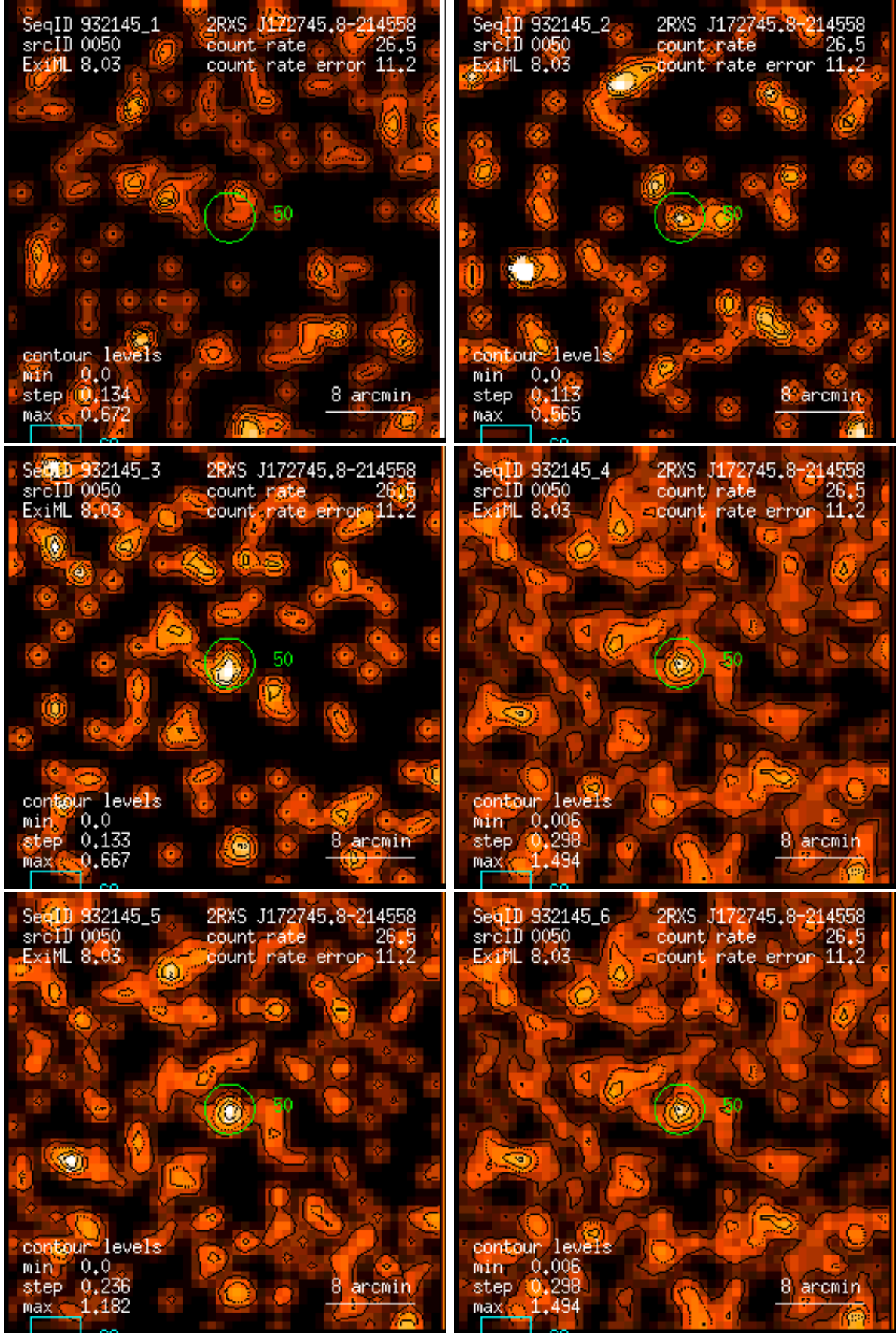
Figure 50: RASS 932145: detection 0050: band rate images, Gaussian filter: (1) PSPC channels 11 – 41, (2) 52 – 90, (3) 91 – 201, (4) 11 – 235, (5) 52 – 201, (6) 11 – 201. Broad band rates in counts/ks. Band rate contour levels in counts/ks/arcmin 2 .
