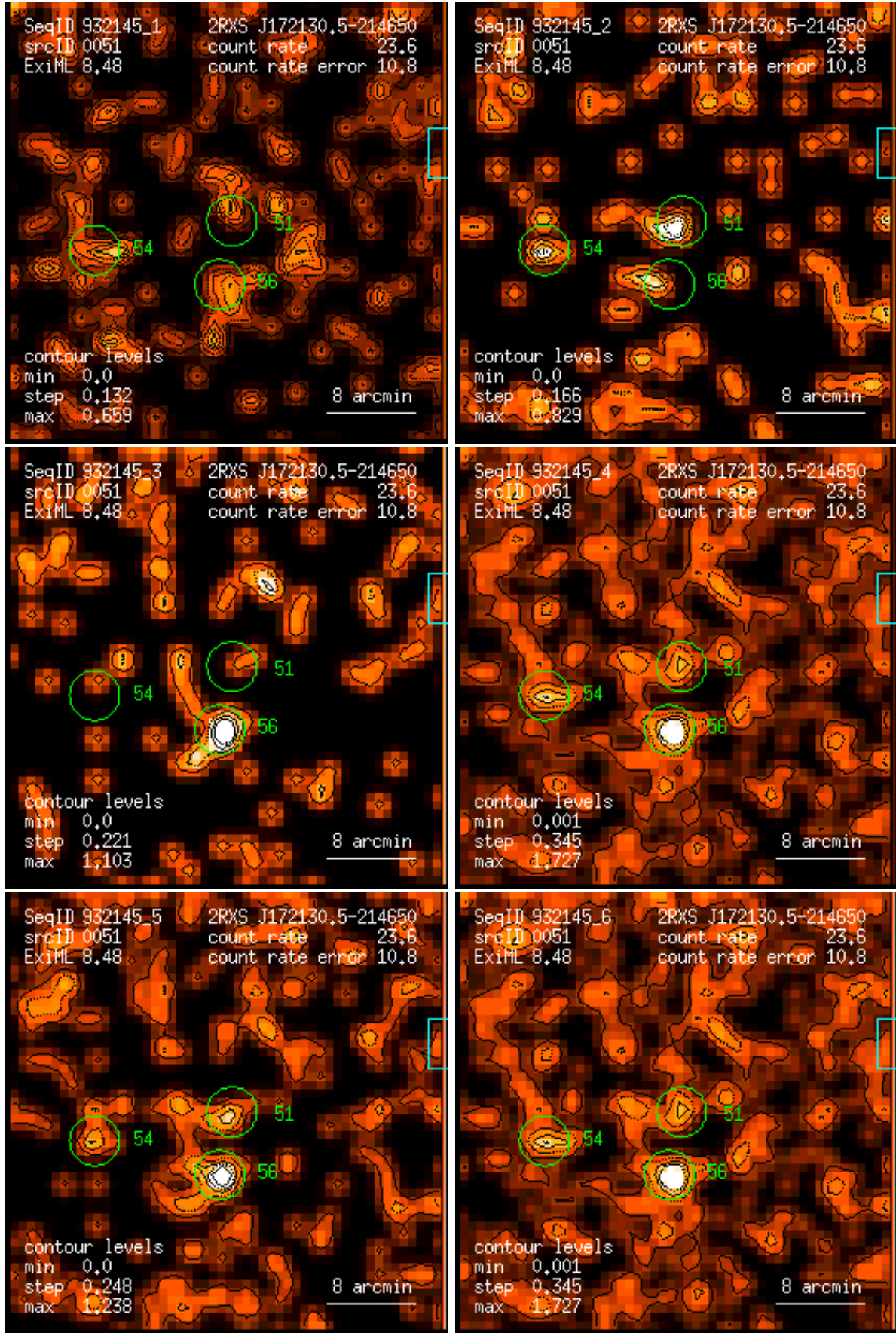
Figure 51: RASS 932145: detection 0051: band rate images, Gaussian filter: (1) PSPC channels 11 – 41, (2) 52 – 90, (3) 91 – 201, (4) 11 – 235, (5) 52 – 201, (6) 11 – 201. Broad band rates in counts/ks. Band rate contour levels in counts/ks/arcmin 2 .
