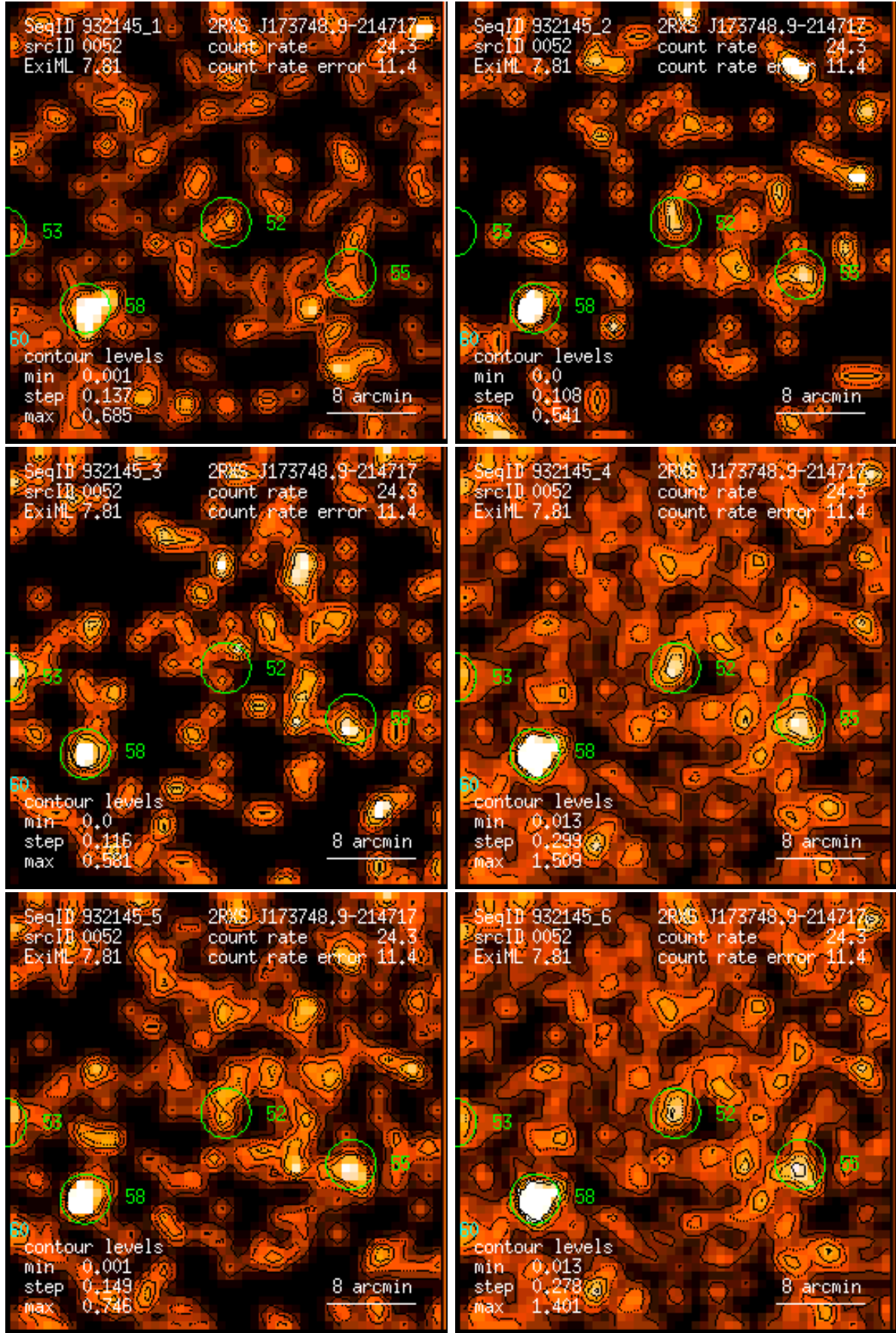
Figure 52: RASS 932145: detection 0052: band rate images, Gaussian filter: (1) PSPC channels 11 – 41, (2) 52 – 90, (3) 91 – 201, (4) 11 – 235, (5) 52 – 201, (6) 11 – 201. Broad band rates in counts/ks. Band rate contour levels in counts/ks/arcmin 2 .
