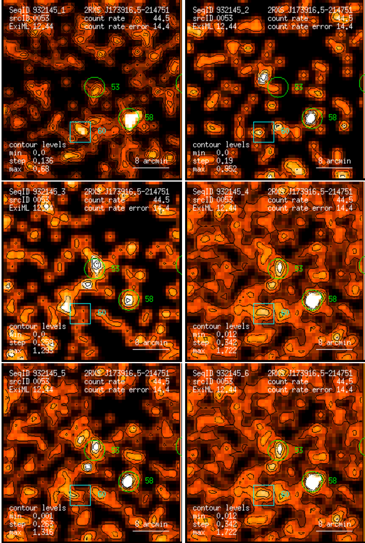
Figure 53: RASS 932145: detection 0053: band rate images, Gaussian filter: (1) PSPC channels 11 – 41, (2) 52 – 90, (3) 91 – 201, (4) 11 – 235, (5) 52 – 201, (6) 11 – 201. Broad band rates in counts/ks. Band rate contour levels in counts/ks/arcmin 2 .
