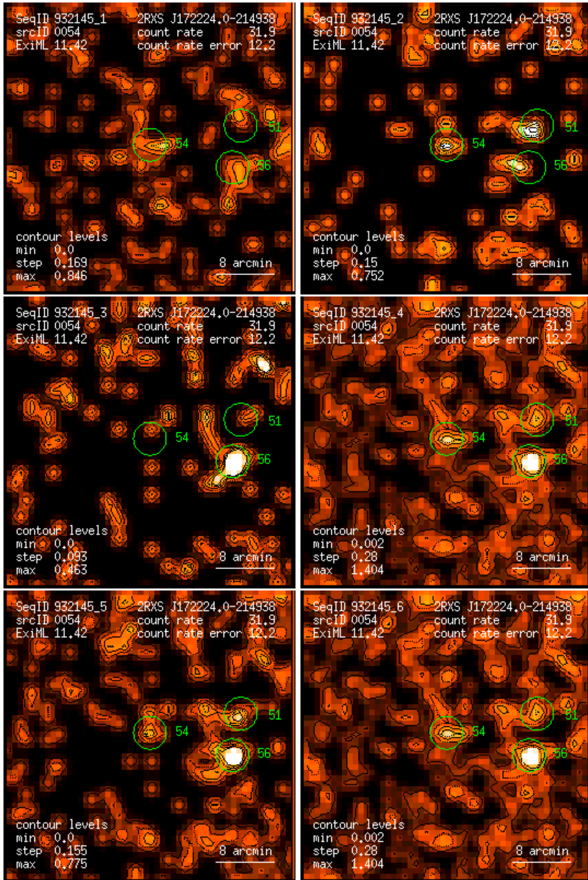
Figure 54: RASS 932145: detection 0054: band rate images, Gaussian filter: (1) PSPC channels 11 – 41, (2) 52 – 90, (3) 91 – 201, (4) 11 – 235, (5) 52 – 201, (6) 11 – 201. Broad band rates in counts/ks. Band rate contour levels in counts/ks/arcmin 2 .
