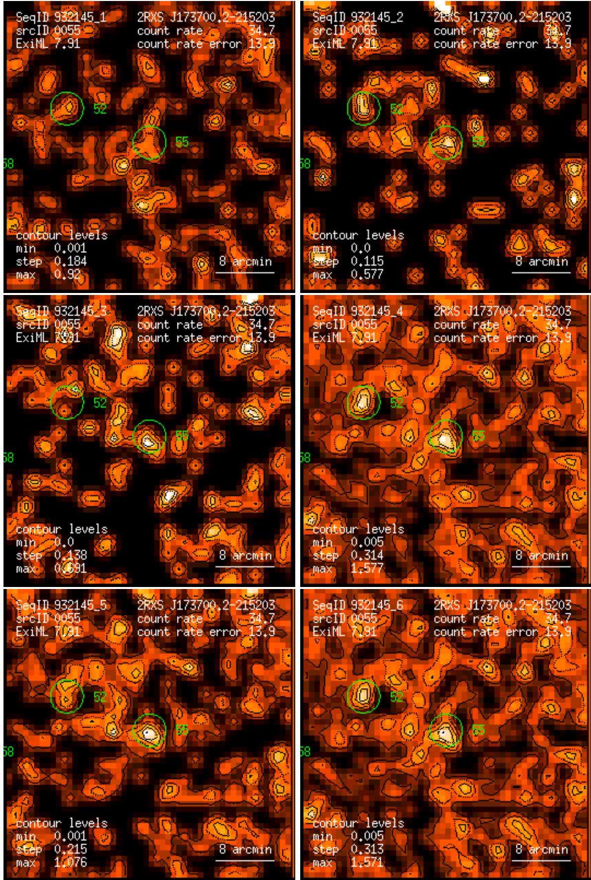
Figure 55: RASS 932145: detection 0055: band rate images, Gaussian filter: (1) PSPC channels 11 – 41, (2) 52 – 90, (3) 91 – 201, (4) 11 – 235, (5) 52 – 201, (6) 11 – 201. Broad band rates in counts/ks. Band rate contour levels in counts/ks/arcmin 2 .
