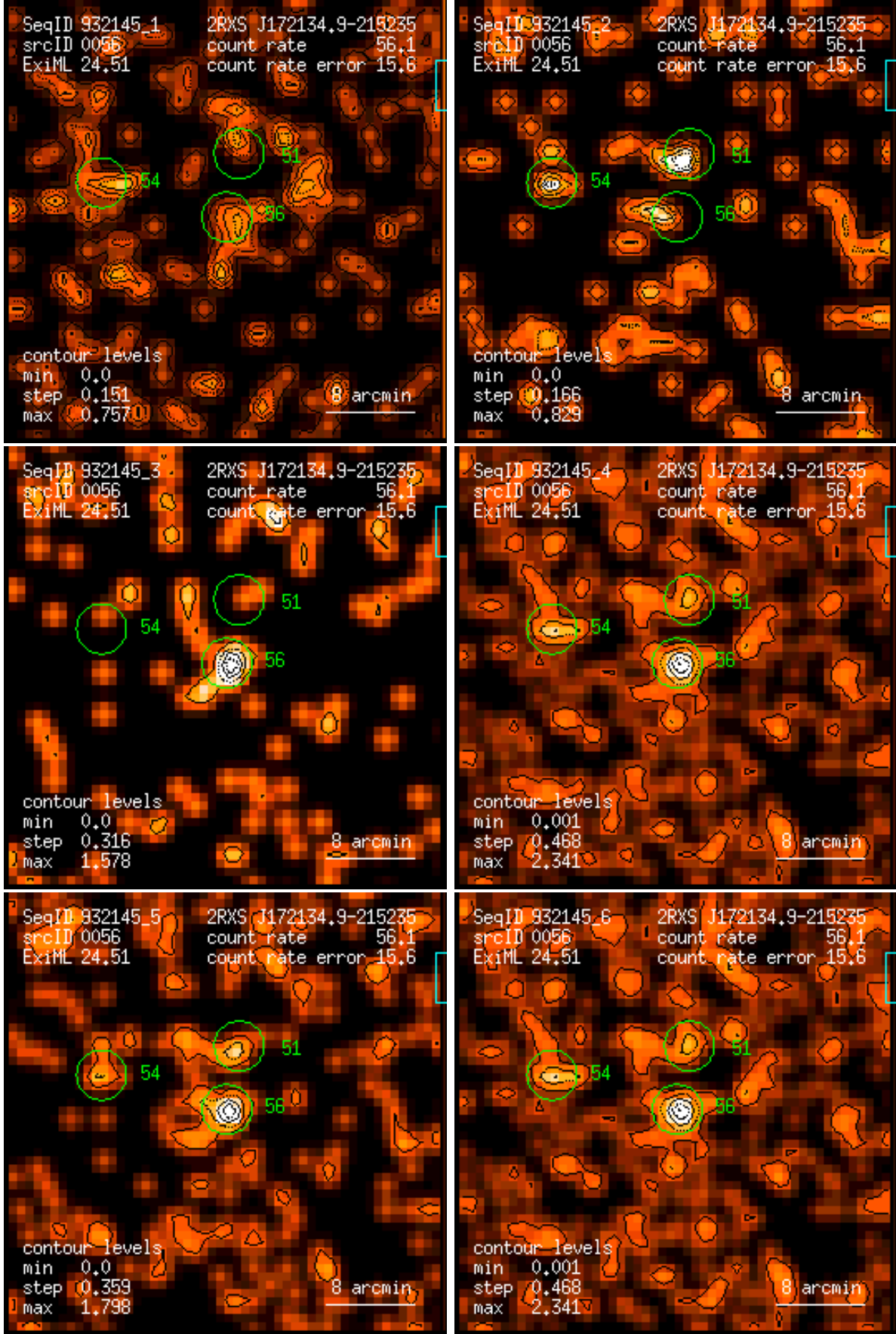
Figure 56: RASS 932145: detection 0056: band rate images, Gaussian filter: (1) PSPC channels 11 – 41, (2) 52 – 90, (3) 91 – 201, (4) 11 – 235, (5) 52 – 201, (6) 11 – 201. Broad band rates in counts/ks. Band rate contour levels in counts/ks/arcmin 2 .
