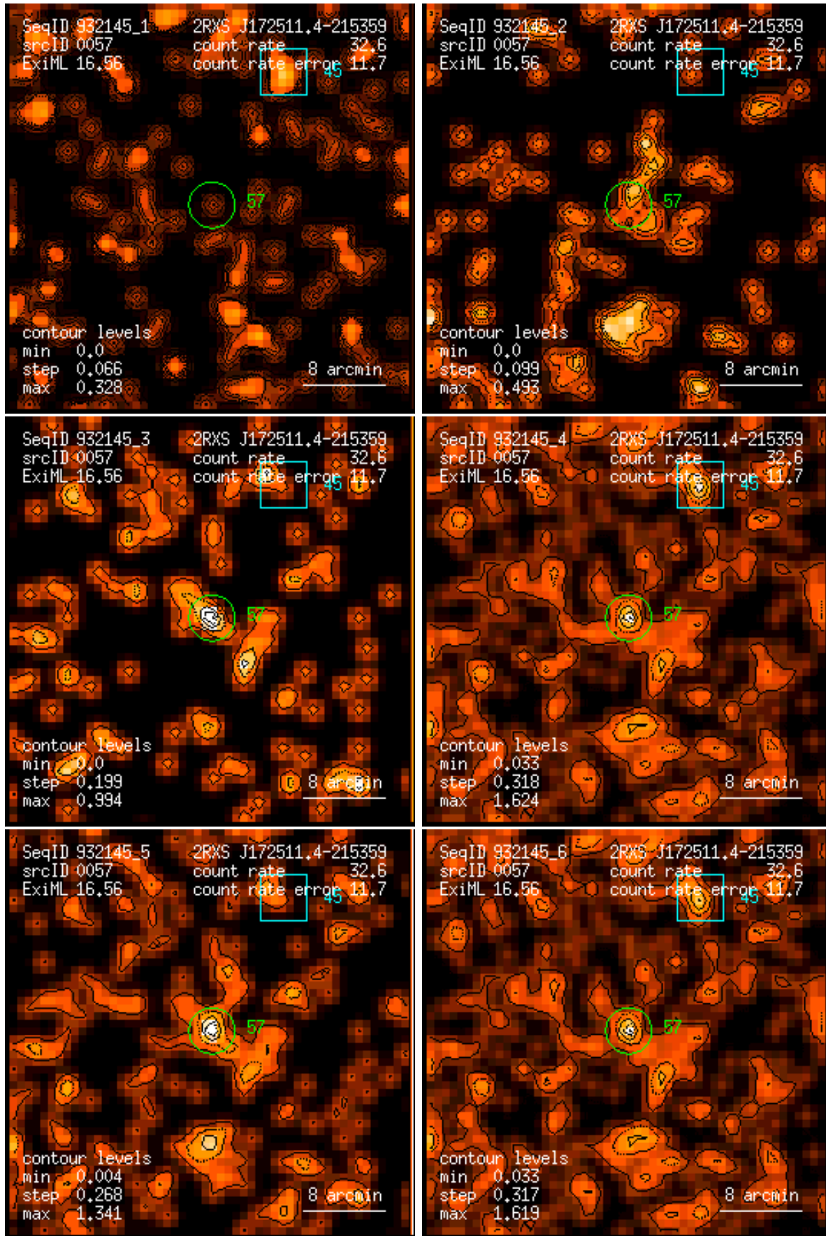
Figure 57: RASS 932145: detection 0057: band rate images, Gaussian filter: (1) PSPC channels 11 – 41, (2) 52 – 90, (3) 91 – 201, (4) 11 – 235, (5) 52 – 201, (6) 11 – 201. Broad band rates in counts/ks. Band rate contour levels in counts/ks/arcmin 2 .
