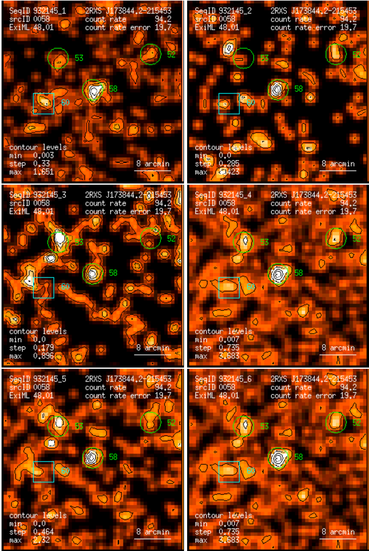
Figure 58: RASS 932145: detection 0058: band rate images, Gaussian filter: (1) PSPC channels 11 – 41, (2) 52 – 90, (3) 91 – 201, (4) 11 – 235, (5) 52 – 201, (6) 11 – 201. Broad band rates in counts/ks. Band rate contour levels in counts/ks/arcmin 2 .
