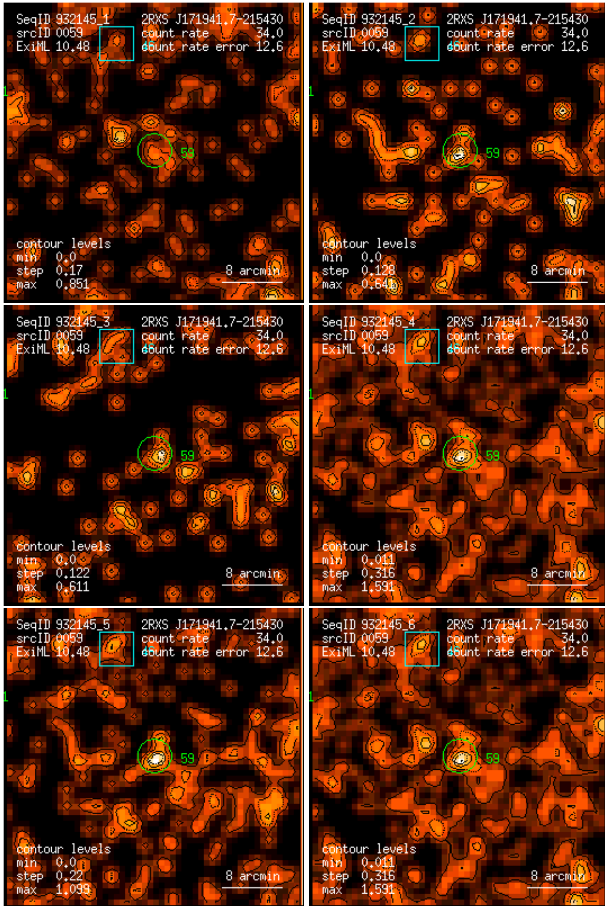
Figure 59: RASS 932145: detection 0059: band rate images, Gaussian filter: (1) PSPC channels 11 – 41, (2) 52 – 90, (3) 91 – 201, (4) 11 – 235, (5) 52 – 201, (6) 11 – 201. Broad band rates in counts/ks. Band rate contour levels in counts/ks/arcmin 2 .
