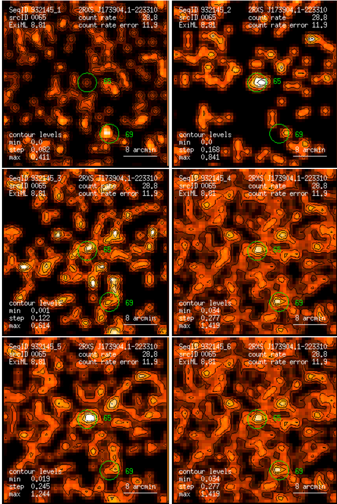
Figure 65: RASS 932145: detection 0065: band rate images, Gaussian filter: (1) PSPC channels 11 – 41, (2) 52 – 90, (3) 91 – 201, (4) 11 – 235, (5) 52 – 201, (6) 11 – 201. Broad band rates in counts/ks. Band rate contour levels in counts/ks/arcmin 2 .
