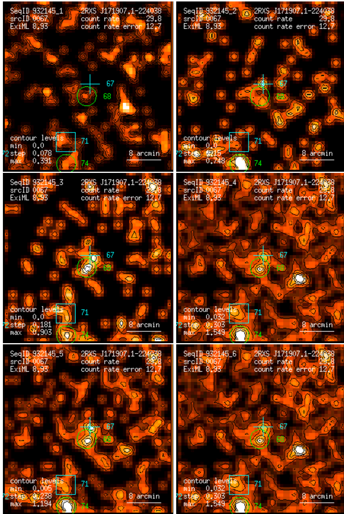
Figure 67: RASS 932145: detection 0067: band rate images, Gaussian filter: (1) PSPC channels 11 – 41, (2) 52 – 90, (3) 91 – 201, (4) 11 – 235, (5) 52 – 201, (6) 11 – 201. Broad band rates in counts/ks. Band rate contour levels in counts/ks/arcmin 2 .
