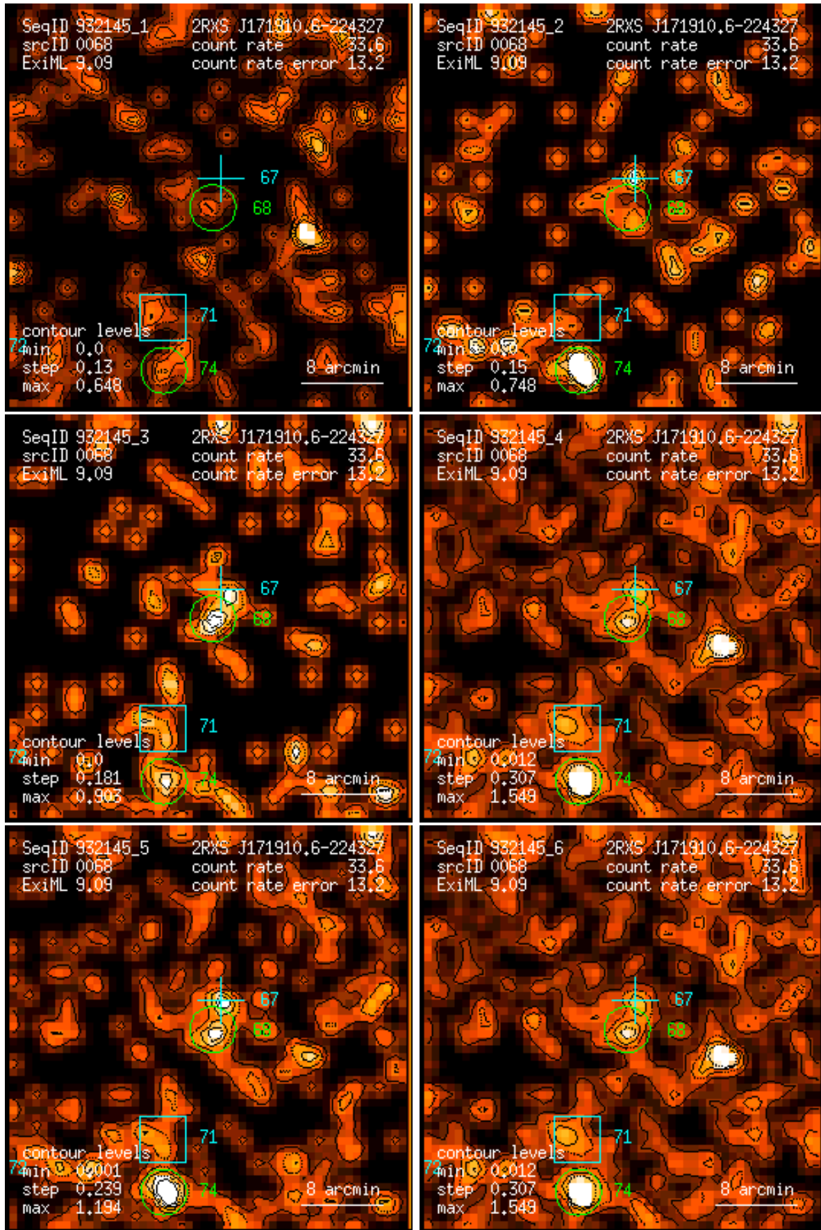
Figure 68: RASS 932145: detection 0068: band rate images, Gaussian filter: (1) PSPC channels 11 – 41, (2) 52 – 90, (3) 91 – 201, (4) 11 – 235, (5) 52 – 201, (6) 11 – 201. Broad band rates in counts/ks. Band rate contour levels in counts/ks/arcmin 2 .
