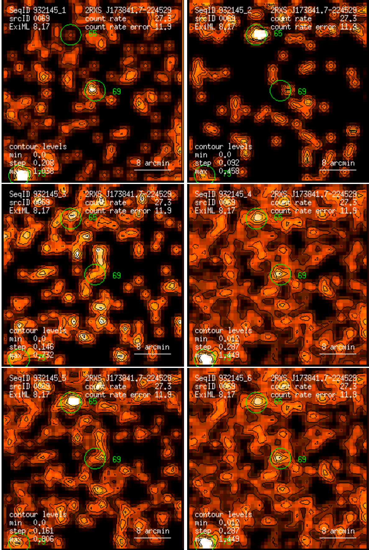
Figure 69: RASS 932145: detection 0069: band rate images, Gaussian filter: (1) PSPC channels 11 – 41, (2) 52 – 90, (3) 91 – 201, (4) 11 – 235, (5) 52 – 201, (6) 11 – 201. Broad band rates in counts/ks. Band rate contour levels in counts/ks/arcmin 2 .
