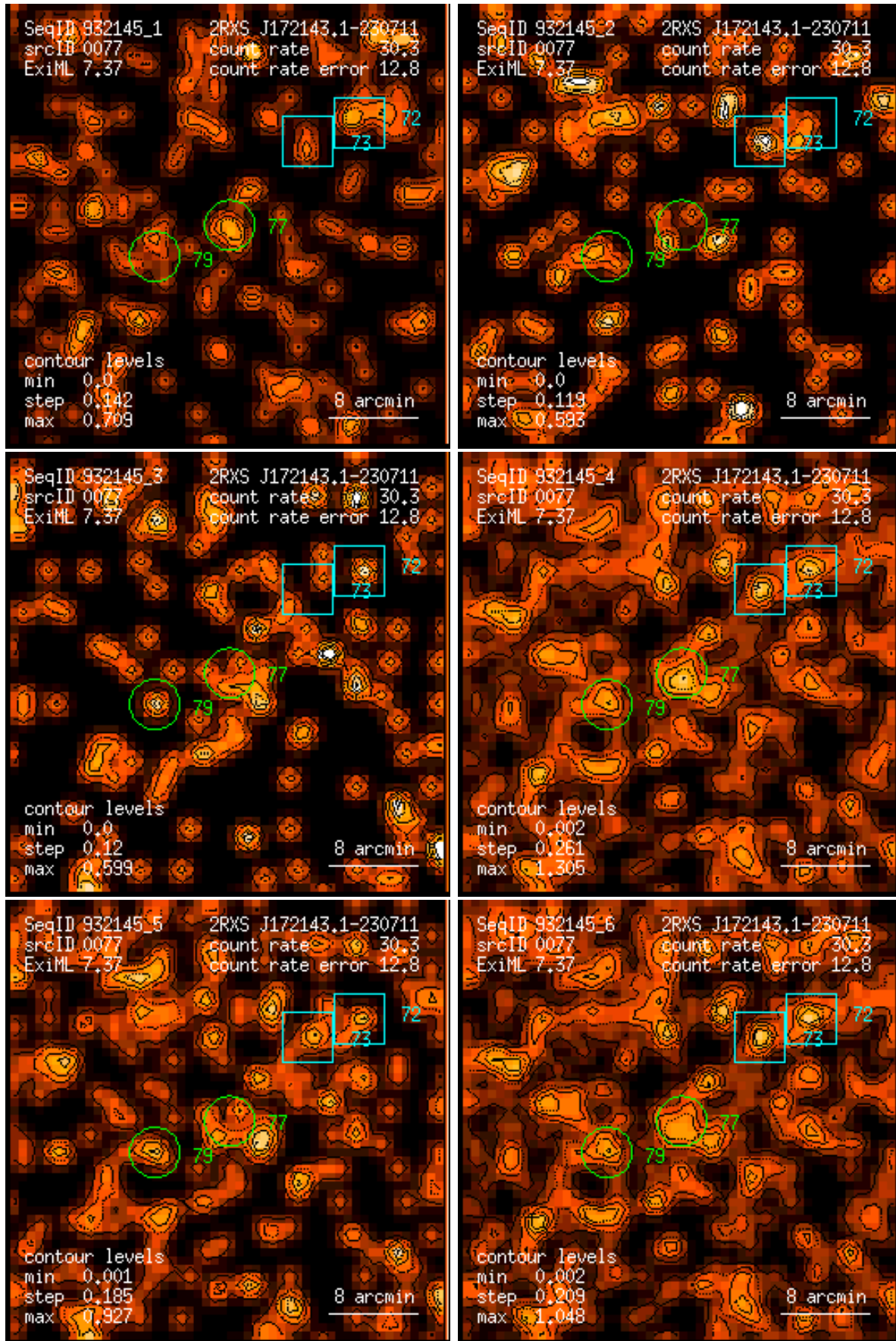
Figure 77: RASS 932145: detection 0077: band rate images, Gaussian filter: (1) PSPC channels 11 – 41, (2) 52 – 90, (3) 91 – 201, (4) 11 – 235, (5) 52 – 201, (6) 11 – 201. Broad band rates in counts/ks. Band rate contour levels in counts/ks/arcmin 2 .
