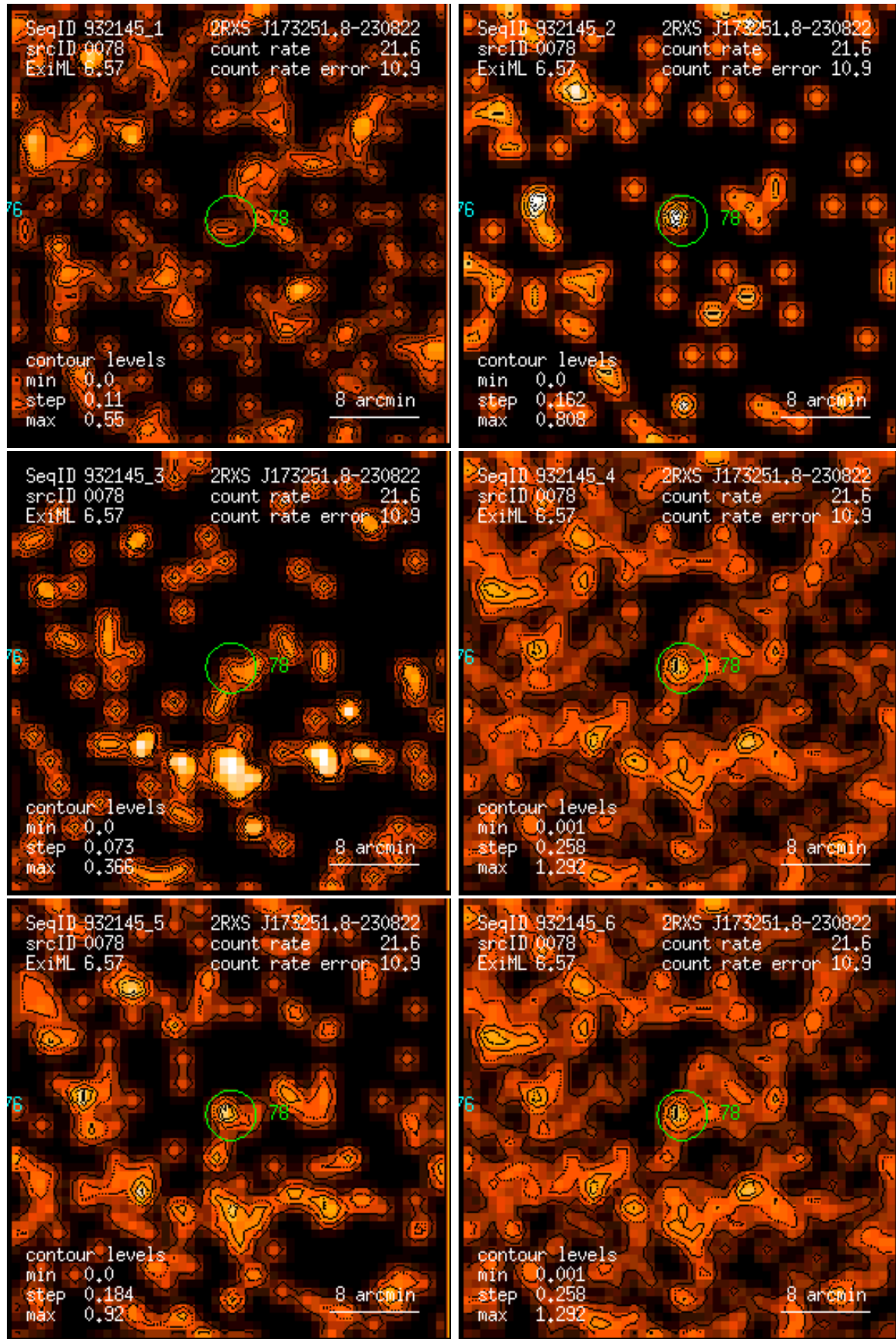
Figure 78: RASS 932145: detection 0078: band rate images, Gaussian filter: (1) PSPC channels 11 – 41, (2) 52 – 90, (3) 91 – 201, (4) 11 – 235, (5) 52 – 201, (6) 11 – 201. Broad band rates in counts/ks. Band rate contour levels in counts/ks/arcmin 2 .
