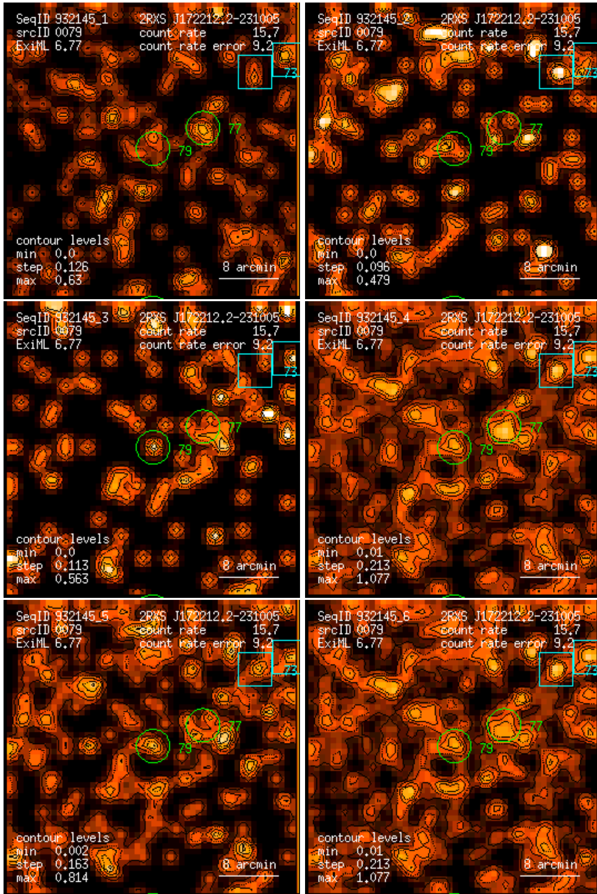
Figure 79: RASS 932145: detection 0079: band rate images, Gaussian filter: (1) PSPC channels 11 – 41, (2) 52 – 90, (3) 91 – 201, (4) 11 – 235, (5) 52 – 201, (6) 11 – 201. Broad band rates in counts/ks. Band rate contour levels in counts/ks/arcmin 2 .
