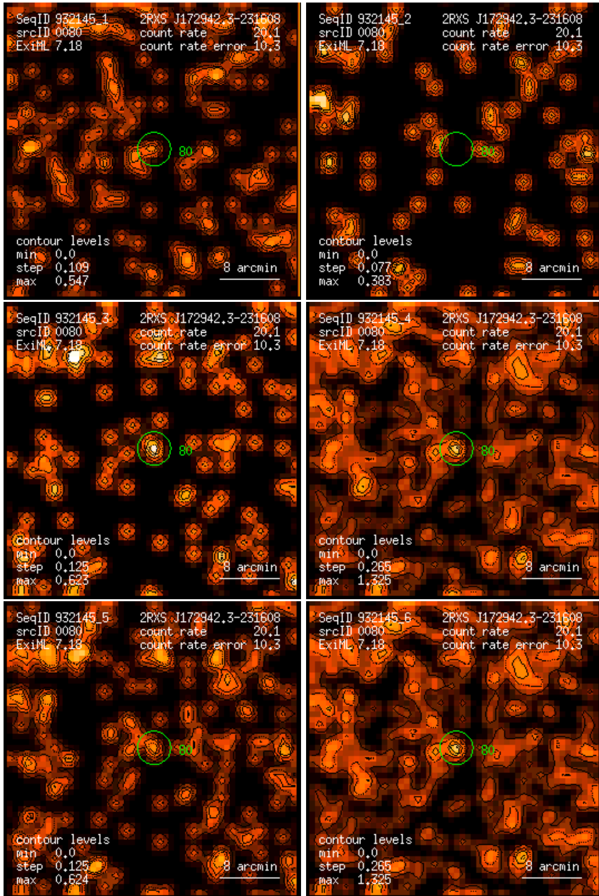
Figure 80: RASS 932145: detection 0080: band rate images, Gaussian filter: (1) PSPC channels 11 – 41, (2) 52 – 90, (3) 91 – 201, (4) 11 – 235, (5) 52 – 201, (6) 11 – 201. Broad band rates in counts/ks. Band rate contour levels in counts/ks/arcmin 2 .
